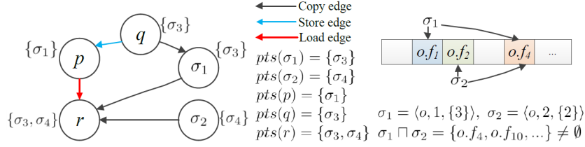
Fig. 8: Resolving \text{Store } p \xleftarrow{\text{Store}} q and \text{Load } r \xleftarrow{\text{Load}} p for overlapping SFRs
