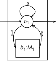
(a) A context-free grammar and its equivalent recursive state machine.
