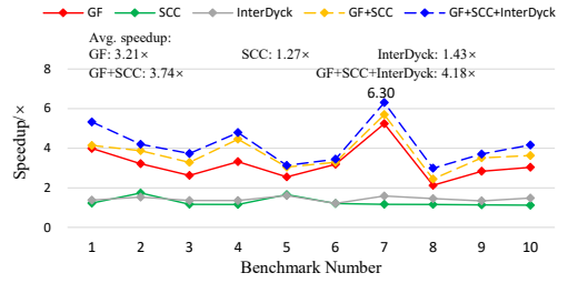
(b) Field-sensitive alias analysis.
