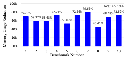
(b) Field-sensitive alias analysis.
