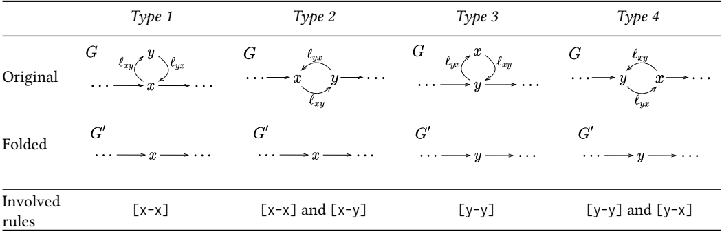
Fig. 7. Four basic types of xy -FEQ classes, where each type contains at most one xy -subpath. For simplicity, we only draw one edge from x to y and one edge from y to x .
