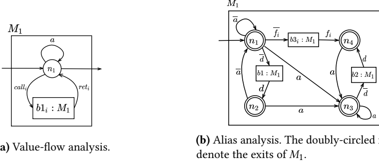
Fig. 9. RSMs for context-sensitive value-flow analysis and field-sensitive alias analysis.
