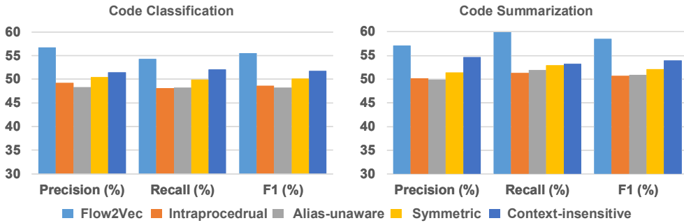
Fig. 11. Ablation analysis for inter-procedural analysis, pointer aliases, asymmetric transitivity and context-sensitivity.
