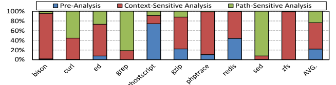
Figure 11: Percentage distribution of CRED’s analysis times.
