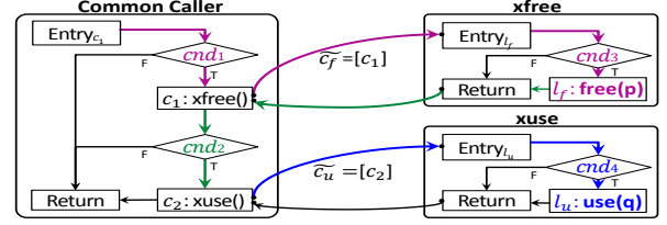
Figure 9: Adding path guards to calling contexts in [PAT-R].
