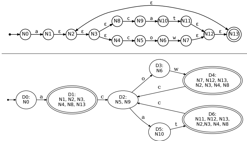
Figure 3.4: Converting an NFA to a DFA via Subset Construction
