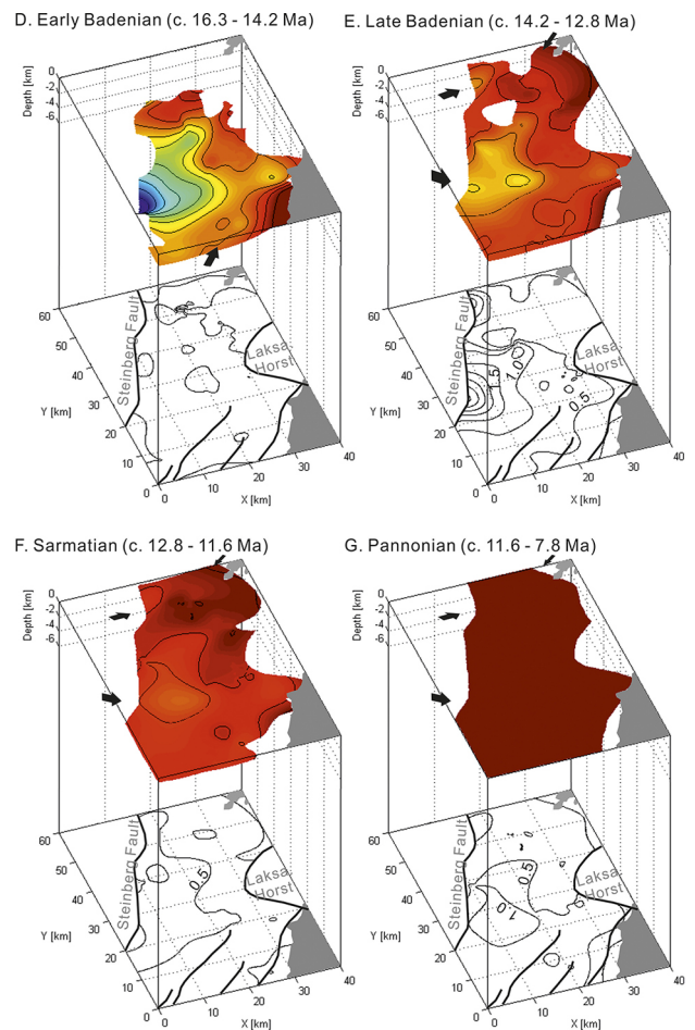
Figure 7: 3D sediment distribution surfaces (above) and sediment thickness isopach maps (below) of the Middle - Late Miocene visualized in the study area; D: early Badenian (c. 16.3 – 14.2 Ma), E: late Badenian (c. 14.2 – 12.8 Ma), F: Sarmatian (c. 12.8 – 11.6 Ma), and G: Pannonian (c. 11.6 – 7.8 Ma). The major faults and contour lines (0.5 km) are shown with black solid lines in the maps. Direction of sediment supply is from Sauer et al. (1992). The top depth of the Pannonian unit is assumed as 0 km.
