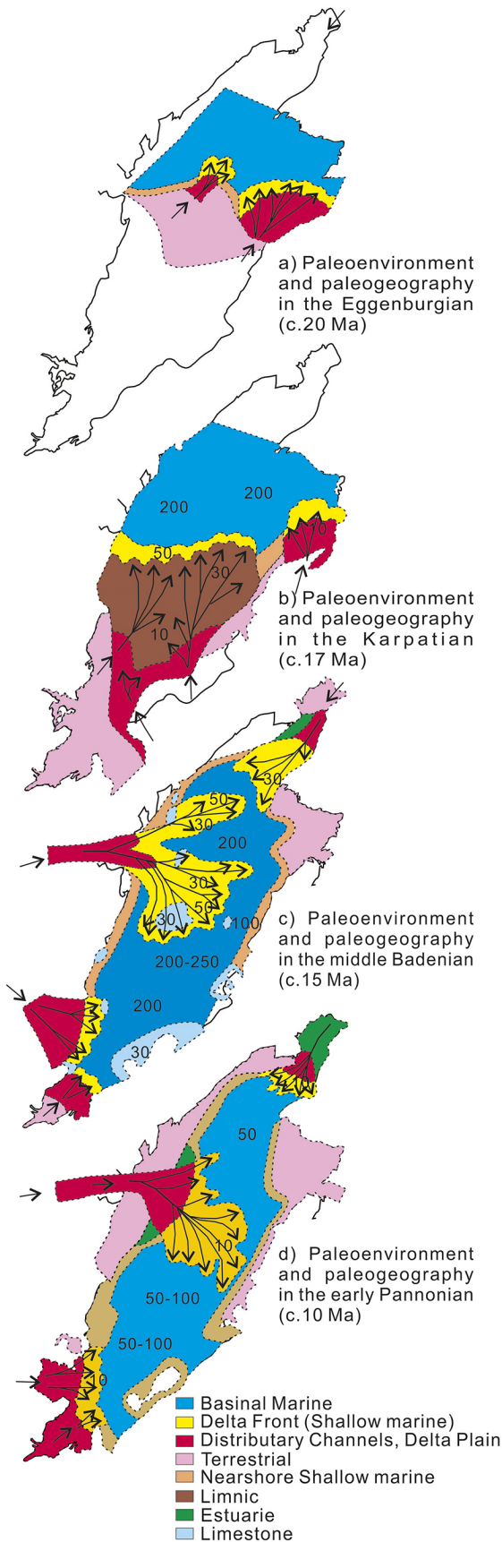
Figure 4: Paleoenvironment and paleogeographic models of the Vienna Basin (revised from Sauer et al., 1992); a) Eggenburgian (c. 20 Ma), b) Karpatian (c. 17 Ma), c) middle Badenian (c. 15 Ma), and d) early Pannonian (c. 10 Ma). Numbers are indicating the paleowater depth.
