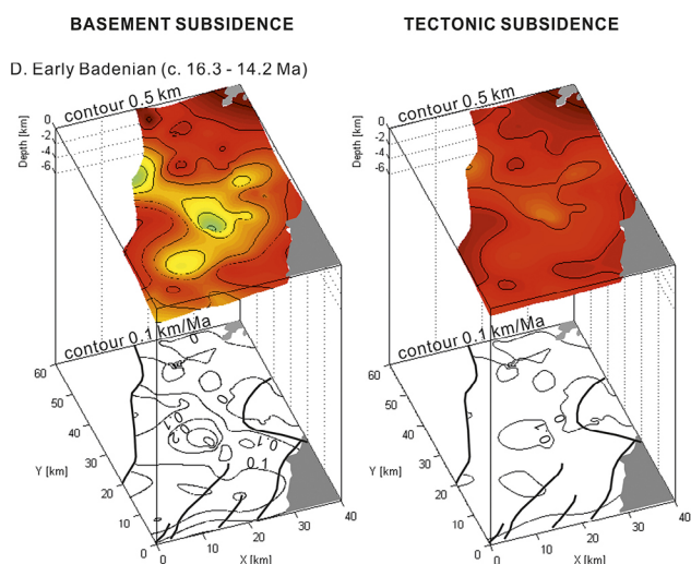
Figure 11: 3D subsidence depth (above) and subsidence rate (below) maps of the basement subsidence (left) and tectonic subsidence (right) visualized in the study area; D: early Badenian (c. 16.3 – 14.2 Ma) and E: late Badenian (c. 14.2 – 12.8 Ma). The major faults are shown with black solid lines in the rate map.
