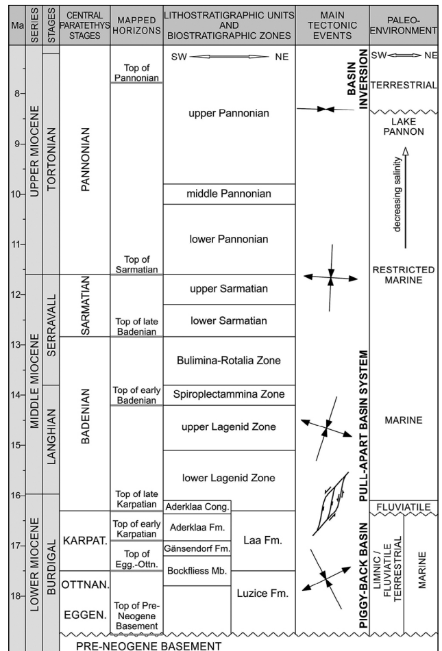
Figure 2: Stratigraphy and evolution of the Vienna Basin in the Miocene (Decker, 1996; Fodor, 1995; Hohenegger et al., 2014; Hölzel et al., 2010; Peresson and Decker, 1997a; Piller et al., 2007; Wagrreich and Schmid, 2002). Horizons mapped in this study are: top of the Pre-Neogene Basement, top of the Eggenburgian-Ottangian, top of the early Karpatian, top of the late Karpatian, top of the early Badenian, top of the late Badenian, top of the Sarmatian, and top of the Pannonian.
