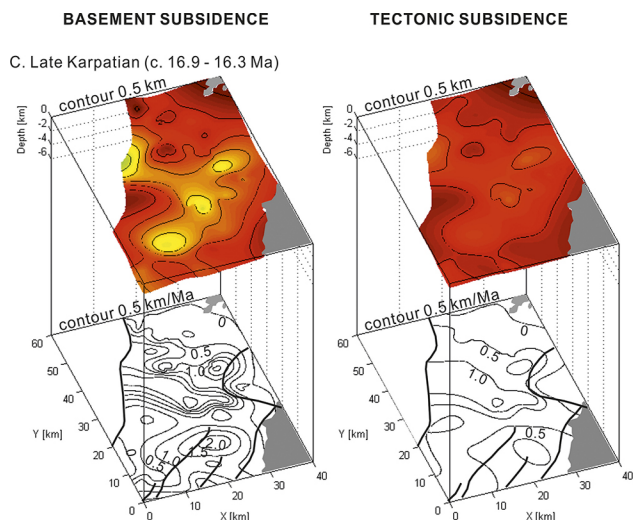
Figure 10: 3D subsidence depth (above) and subsidence rate (below) maps of the basement subsidence (left) and tectonic subsidence (right) visualized in the study area; C: late Karpatian (c. 16.9 – 16.3 Ma). The major faults are shown with black solid lines in the rate map.
