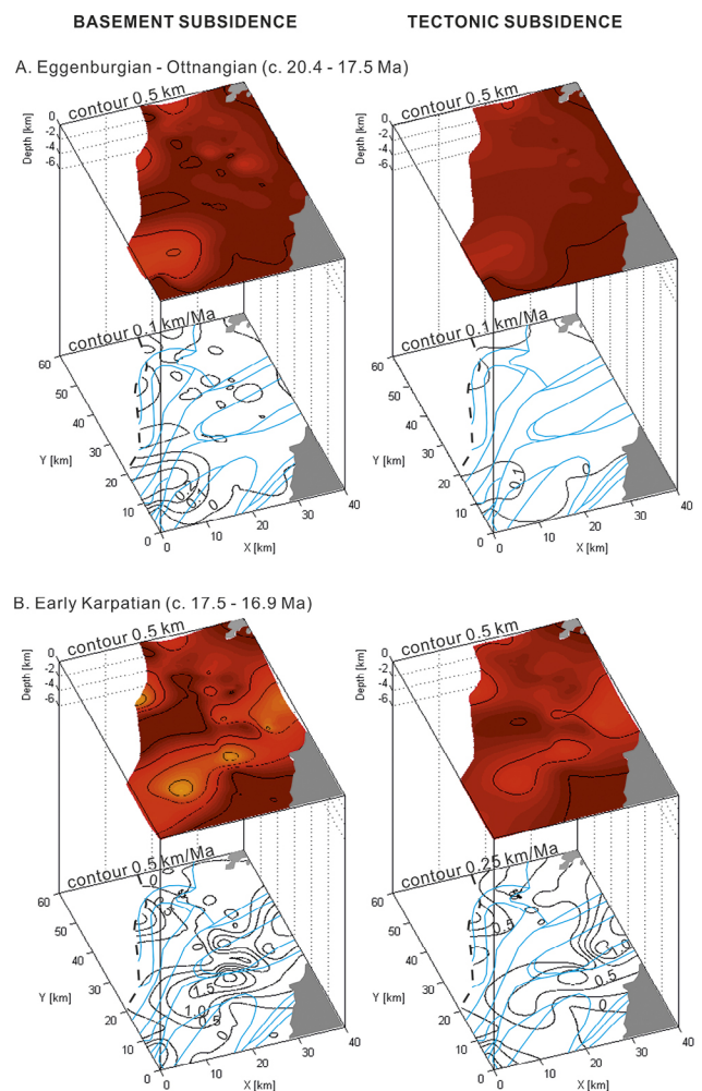
Figure 9: 3D subsidence depth (above) and subsidence rate (below) maps of the basement subsidence (left) and tectonic subsidence (right) visualized in the study area; A: Eggenburgian-Ottngian (c. 20.4 – 17.5 Ma) and B: early Karpatian (17.5 – 16.9 Ma). The Alpine-Carpathian thrust nappe borders are shown with blue solid lines and the location of the Steinberg fault with black broken lines.
