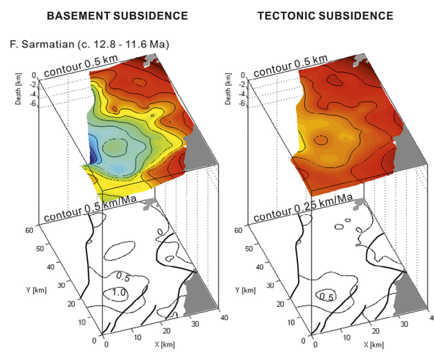
Figure 12: 3D subsidence depth (above) and subsidence rate (below) maps of the basement subsidence (left) and tectonic subsidence (right) visualized in the study area; F: Sarmatian (c. 12.8 – 11.6 Ma) and G: Pannonian (c. 11.6 – 7.8 Ma). The major faults are shown with black solid lines in the rate map.
