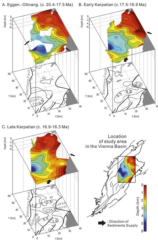
Figure 6: 3D sediment distribution surfaces (above) and sediment thickness isopach maps (below) of the Early Miocene visualized in the study area; A: Eggenburgian-Ottangian (c. 20.4 – 17.5 Ma), B: early Karpatian (c. 17.5 – 16.9 Ma), and C: late Karpatian (c. 16.9 – 16.3 Ma). The major faults and contour lines (0.5 km) are shown with black solid lines in the maps. Direction of sediment supply is from Sauer et al. (1992).
