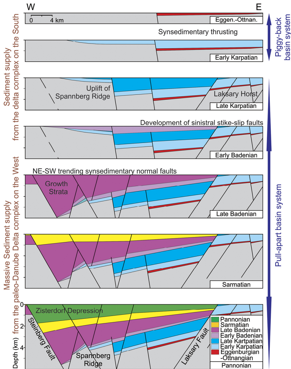
Figure 13: Schematic evolutionary model for sedimentary fill and subsidence evolution of the central Vienna Basin from the Early to Late Miocene in successive cross-sections.
