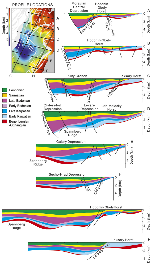
Figure 8: Cross-section profiles across the study area, exported from the cross-section function of BasinVis 1.0. Important structural elements are labeled.
