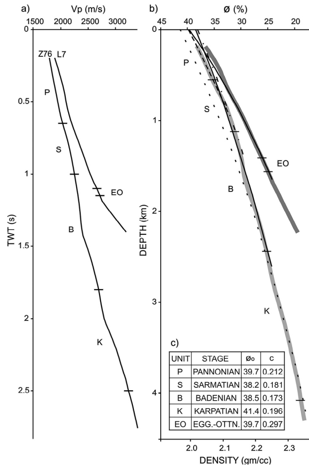
Figure 5: Porosity-depth relation evaluated for the Vienna Basin. a) Seismic velocity-Two Way Time (TWT) curves from locations of two wells (Zavod 76 and Lakšárska Nová Ves 7), b) Porosity and Density-Depth curves with exponential trend lines of each stage, and c) evaluated initial porosity ( \phi_0 ) and coefficient (c) of each stage.
