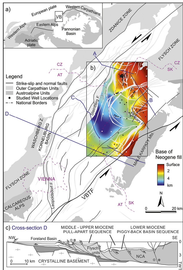
Figure 1: a) Tectonic sketch map of the Vienna Basin located at the junction between the Eastern Alps, the Western Carpathians, and the Pannonian Basin system (revised from Arzmüller et al., 2006; Wessely et al., 1993). b) Study area and depth map of the base Neogene, the latter being a result of this study. Locations of wells (black dots: wells reaching the pre-Neogene basement, gray dots: wells reaching the Miocene basin fill, and white dots: synthetic wells) and cross-sections (A - D) are shown. AT: Austria, SK: Slovakia, CZ: Czech Republic, and VBTF: Vienna Basin transfer fault system. c) Geologic cross-section through the Vienna Basin and the adjacent Alpine Foreland Basin (revised from Beidinger and Decker, 2014).
