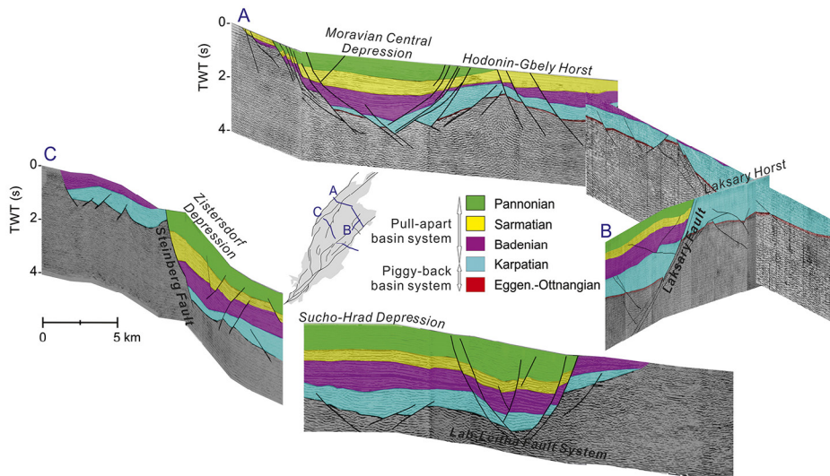
Figure 3: Seismic sections across the study area (see Figure 1 for location). Section A and C were revised from Čekan et al. (1990), and section B was acquired from the archives of the Dionyz Štur Institute, Slovakia. These sections were visualized by Blender which is an open-source 3D computer graphics software.
