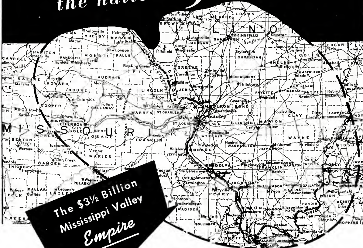
DAYTIME 0.5 MV/M CONTOUR FOR KXOK 630KC 5KW
