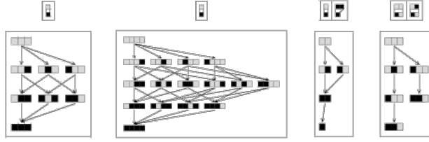
Figure 7: The multiway systems generated by the evolution of three (globally) confluent string substitution systems - the first two evolutions generated by A \rightarrow B , and the last two generated by \{A \rightarrow B, BB \rightarrow B\} and \{AA \rightarrow BA, AB \rightarrow BA\} , respectively. Irrespective of which rewriting path is chosen, the same eventual outcome (i.e. the same normal form) is always reached. Adapted from S. Wolfram, A New Kind of Science , pages 507 and 1037.
