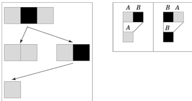
Figure 6: The multiway system generated by the evolution of a (globally) non-confluent string substitution system, \{AB \rightarrow A, BA \rightarrow B\} , starting with the initial condition ABA , in which distinct normal forms are obtained for the two possible rewriting paths. Adapted from S. Wolfram, A New Kind of Science , page 205.
