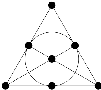
Figure 11: The Fano plane represented using the Steiner system S(2, 3, 7) (historically known as a Steiner triple system, since k = 3 = t + 1 ); the 7 blocks correspond to the 7 lines of the plane, each of which contains exactly 3 points, and with the property that every pair of points lies on exactly one line.
