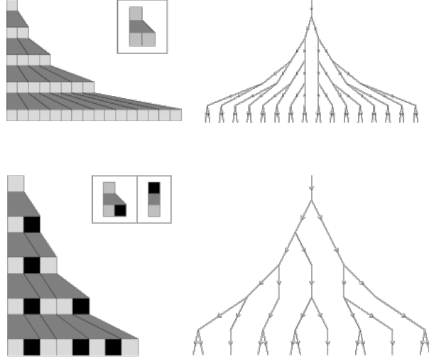
Figure 9: The causal graphs generated by the evolution of two (globally) confluent string substitution systems - A \rightarrow AA and \{A \rightarrow AB, B \rightarrow A\} , respectively. The combinatorial structure of the causal graph is invariant to the choice of multiway system path, and therefore to the choice of rewriting order. Adapted from S. Wolfram, A New Kind of Science , page 500.
