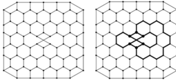
Figure 14: On the left is a trivalent spatial graph containing an irreducible crossing of edges. ON the right is an illustration of how this irreducible crossing is ultimately due to the presence of a non-planar “tangle” this is a subdivision of K_{3,3} . Adapted from S. Wolfram, A New Kind of Science , page 527.
