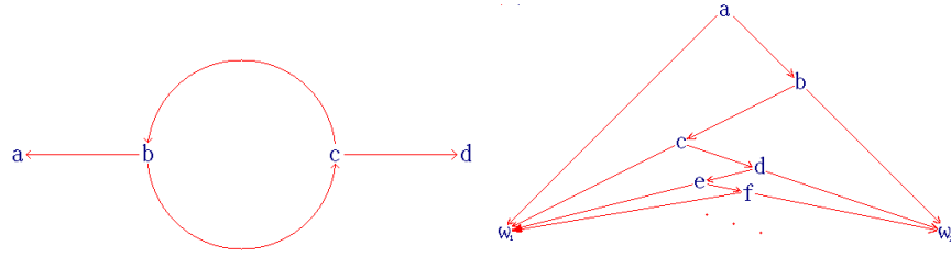
Figure 5: On the left is a locally confluent rewriting system, in which the presence of a cycle allows the system to evade global confluence. On the right is a locally confluent and acyclic rewriting system, in which the presence of an infinite linear rewrite sequence allows the system to evade global confluence in essentially the same way. Images by Jochen Burghardt, distributed under a CC BY-SA 3.0 license.
