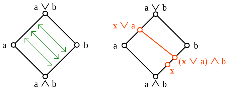
Figure 13: On the left, we see the diamond isomorphism theorem being satisfied for the modular pair (a, b) , since the maps \phi : [a \wedge b] \rightarrow [a, a \vee b] and \psi : [a, a \vee b] \rightarrow [a \wedge b, b] indicated by the green arrows are both bijective and order-preserving, and hence isomorphisms. On the right, we see the failure of the diamond isomorphism theorem for the non-modular pair (a, b) , since the map between (x \vee a) \wedge b and x \vee b is no longer invertible for some x , as shown by the orange line.
