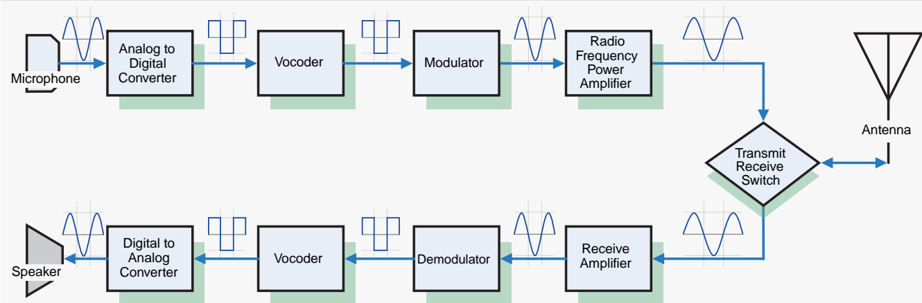
Figure 3.2. Digital Radio
