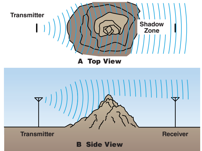
Figure 2.9. Terrain Blocking
