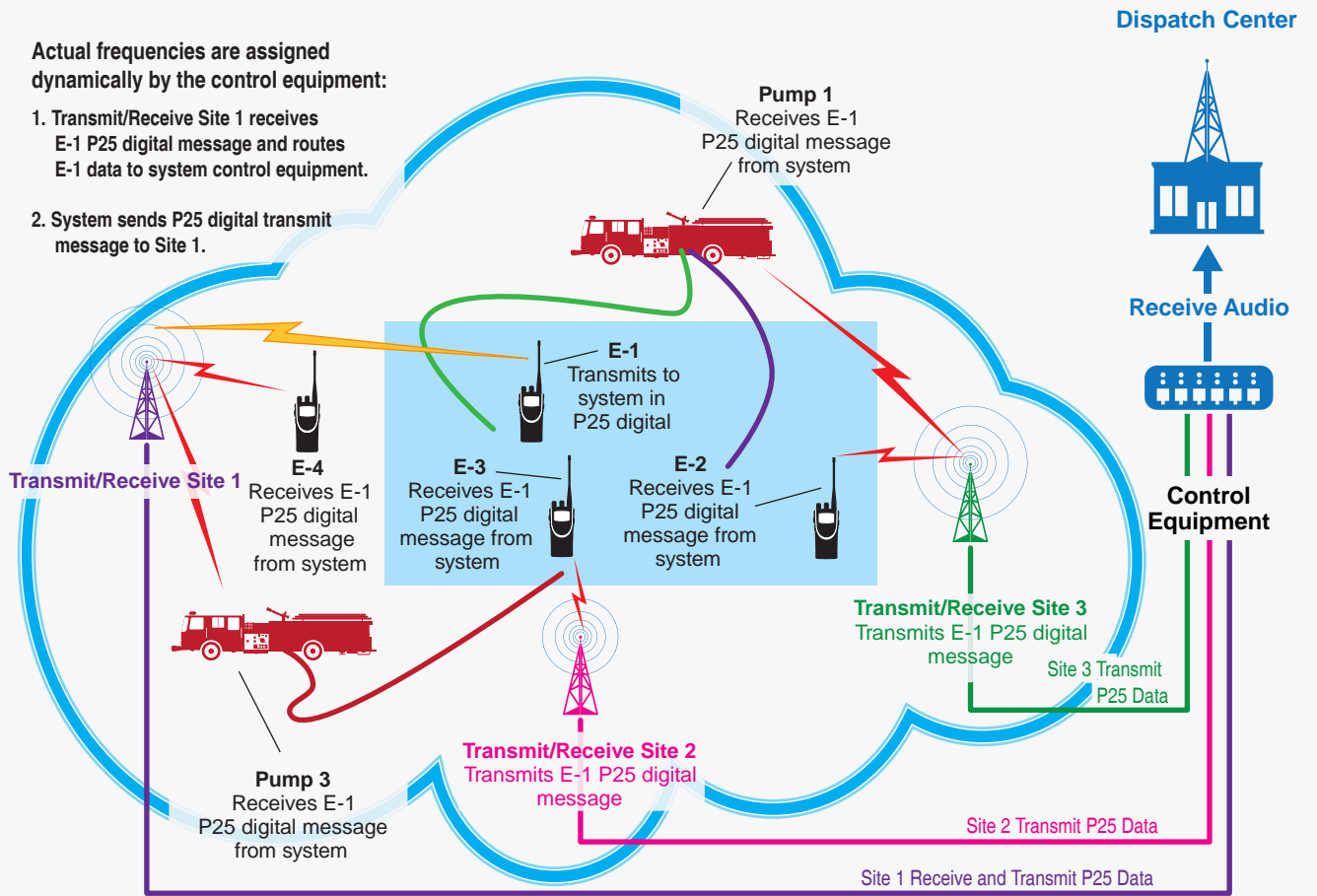
Figure 5.2. Trunked Radio System — Portable Radio Transmit — Fireground Communications
