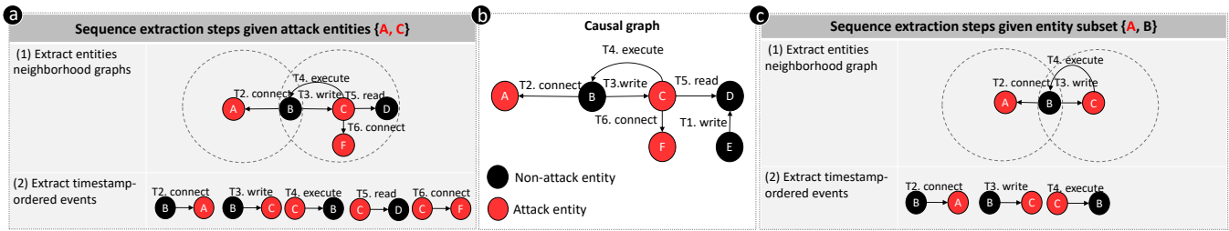
Figure 5: (Middle) An example causal graph to illustrate sequence construction process. (Left) Attack sequence extraction steps. (Right) Non-attack sequence extraction steps.
