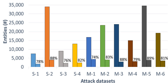
Figure 8: Effectiveness of causal graph optimization of given audit logs for attack investigation. The percentages on the bars show the percentage of the logs reduction.
