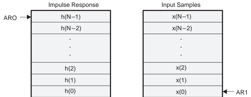
Figure 6–12. Data Structure for FIR Filters
