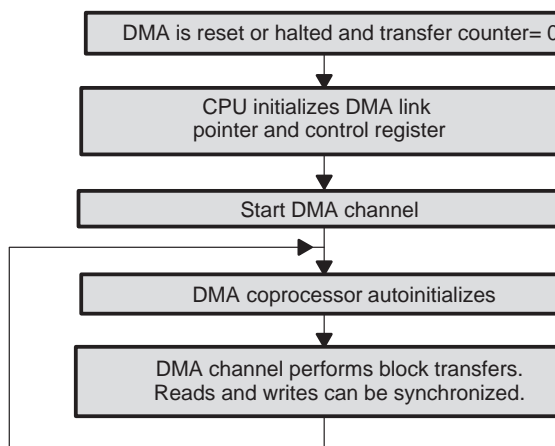
Figure 11–13. DMA Channel Running in Transfer Mode 10 2 (Autoinitialization Method 1a)
