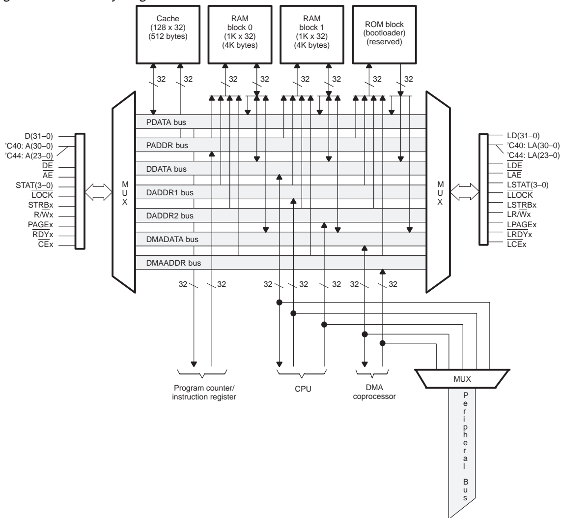
Figure 2–3. Memory Organization
