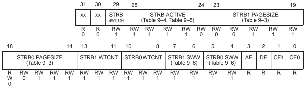
Figure 9–3. Fields in the Memory-Interface Control Registers
