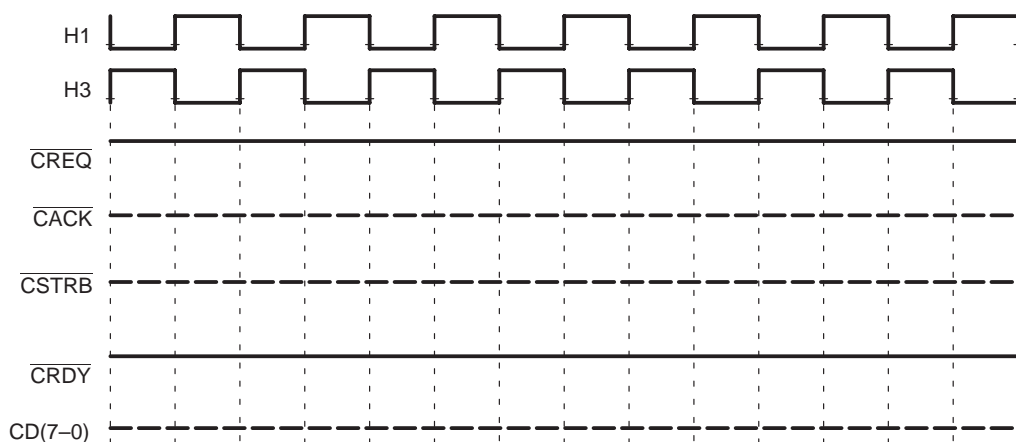
Figure 12–15. Post-Reset State for an Input Port
