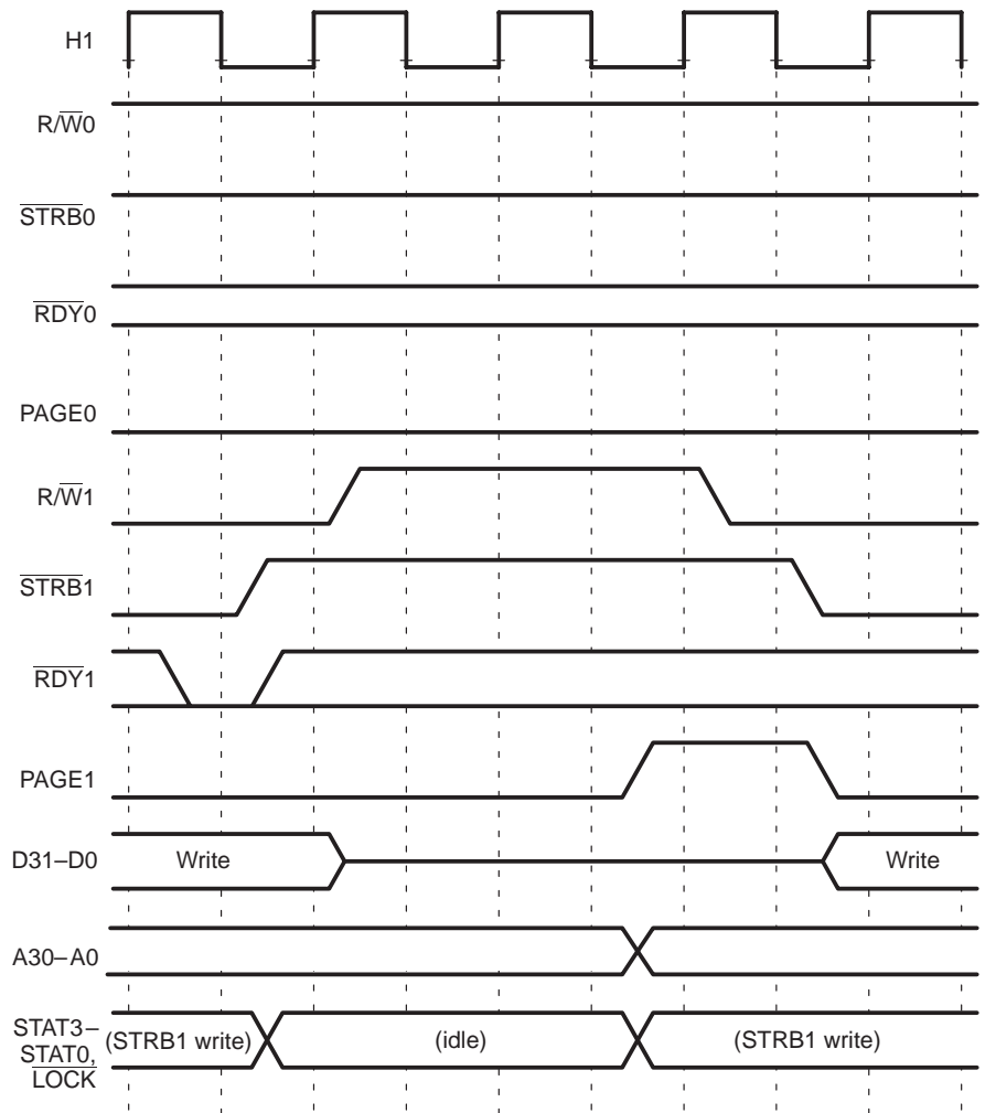
Figure 9–16. Write Same Page, Idle One Cycle, Write Different Page Sequence
