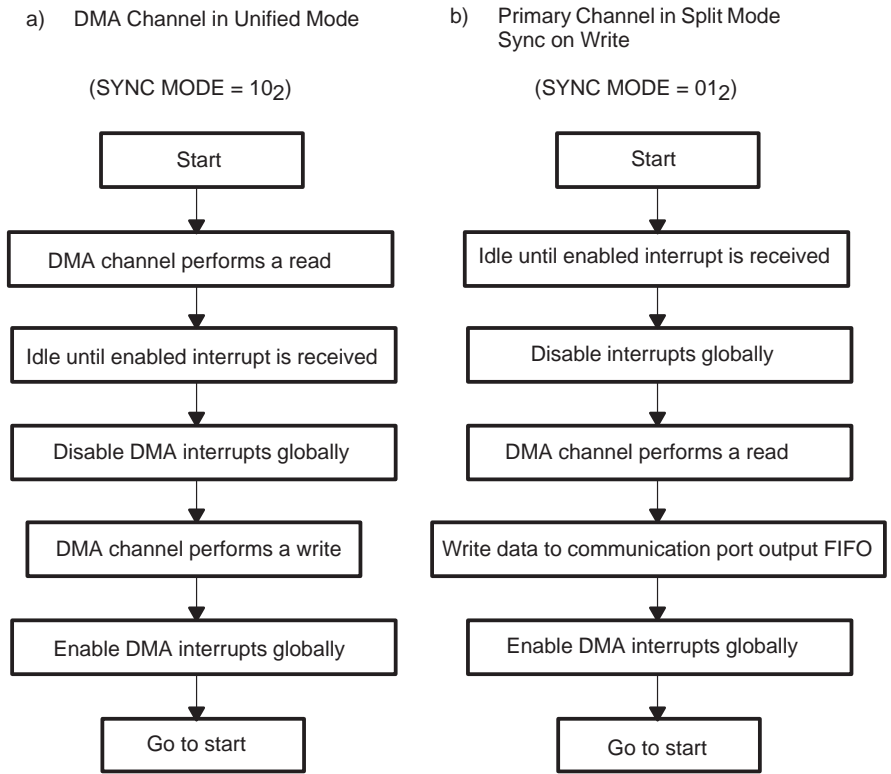
Figure 11–29. DMA Destination Synchronization
