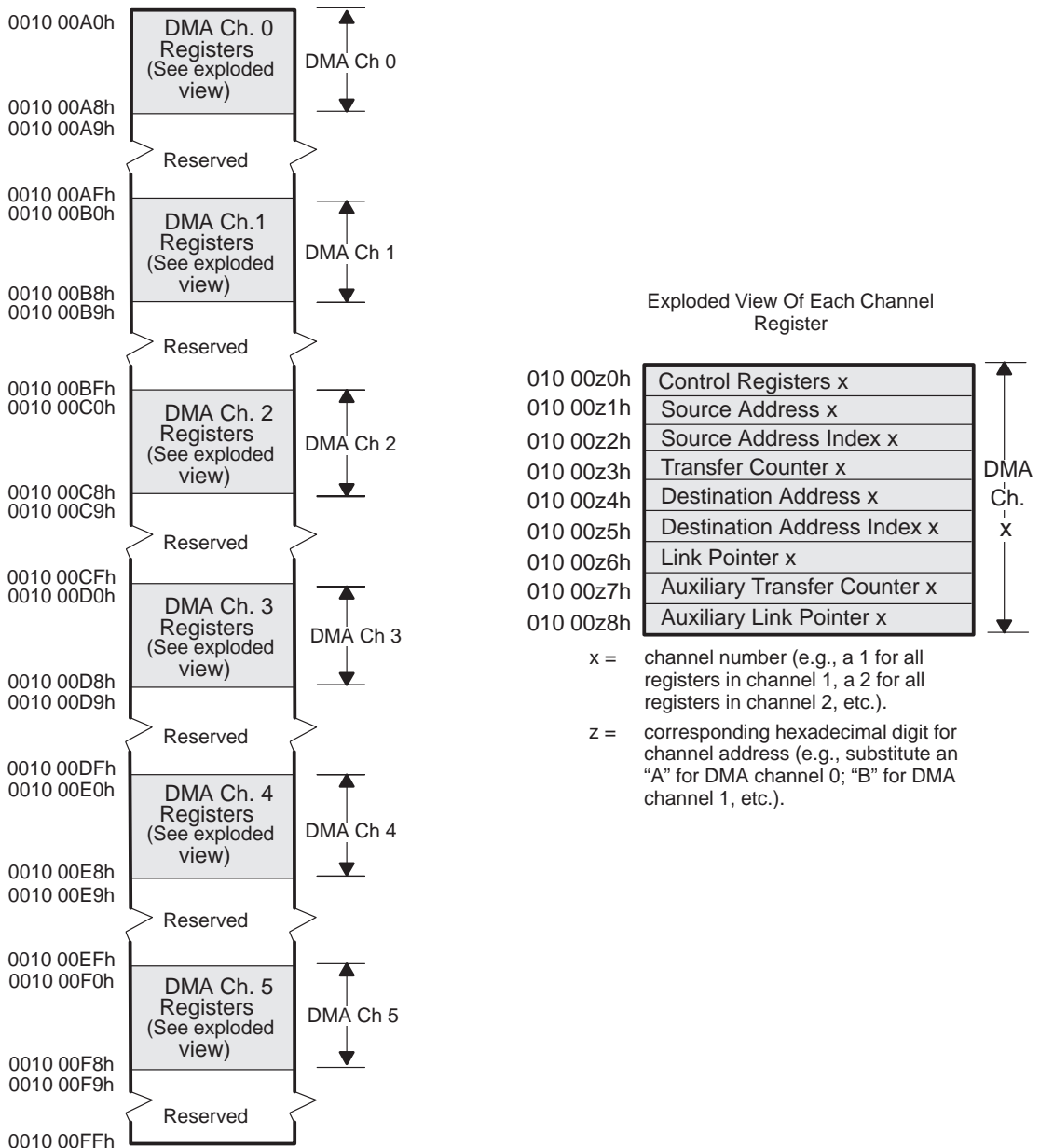
Figure 11–1. DMA Coprocessor Memory Map
