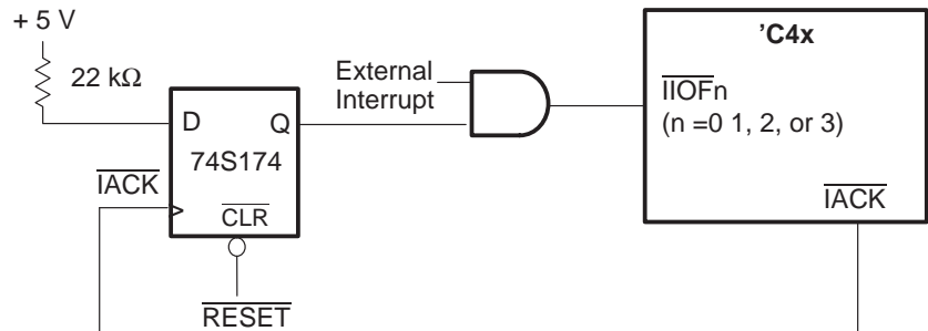
Figure 10-4. Circuit for Generation of a Low IIOF Signal for Bootloader Selection
