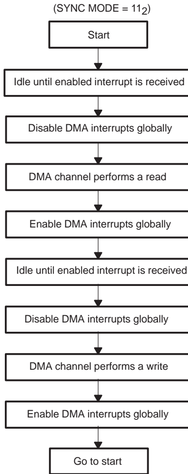
Figure 11–30. Unified Mode DMA Source and Destination Synchronization
