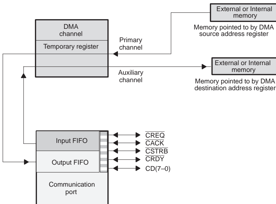
Figure 11–7. Typical Split-Mode DMA Configuration
