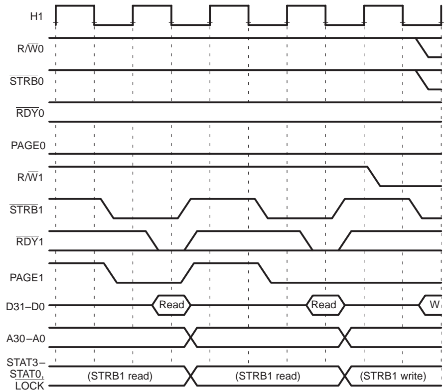
Figure 9–12. Read Different Page, Read Different Page, Write Same Page Sequence
