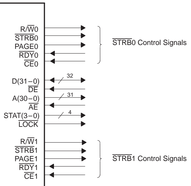
Figure 9–1. Global and Local Memory Interface Control Signals
