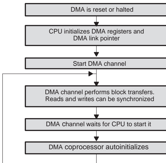
Figure 11–16. DMA Channel Running in Transfer Mode 11 2 (Autoinitialization Method 2b)
