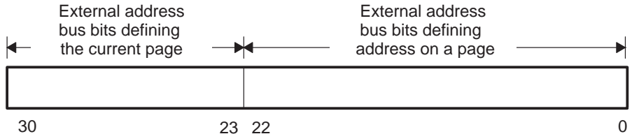
Figure 9–5. \overline{\text{STRB}}_x PAGESIZE Fields Example
