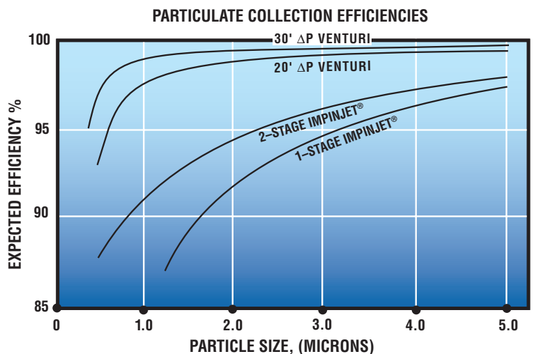
PARTICULATE COLLECTION EFFICIENCIES
