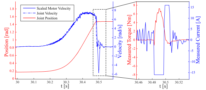
Fig. 10. Joint torque during impulsive collision. The motor velocity is scaled with the gear ratio for plotting purposes.
