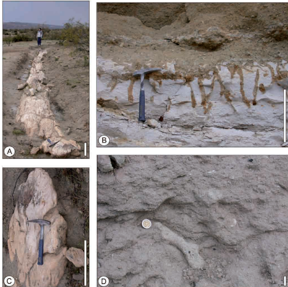
FIGURE 3 | A) Portion of an exposed large trunk of Podocarpoxylon mazzonii . B) View of Glossifungites icnofacies, Thalassinoides sp. with passive filling. Scale bar: 20cm. C) Natural view the fragment wood of Podocarpoxylon mazzonii at Ameghino Petrified Forests. D) Thalassinoides sp. in fine sands. Scale bar: 20cm in A-C; Coin scale: 2.2cm in diameter in D.
