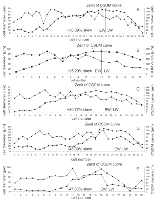
FIGURE 9 | Right-skewed CSDM curves of five growth rings and cell diameters of growth increment. For each ring increment, the percentage of skew for CSDM curves was calculated using Falcon-Lang method (2000a). The distance where CSDM curve reaches the zenith represents the percentage of skew in relation with the total distance between the centre of the CSDM curve to the right of the plot.
