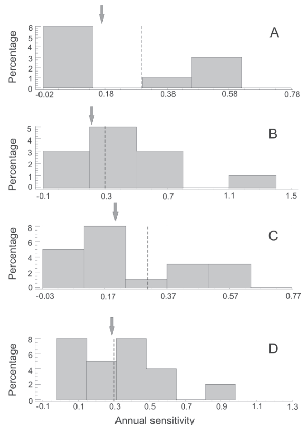
FIGURE 8 | Histograms allowing comparison of variation in the annual sensitivities of selected fossil tree. The arrows indicate position of Mean Sensitivity (MS). Simple dotted line shows the MS: 0.30.
