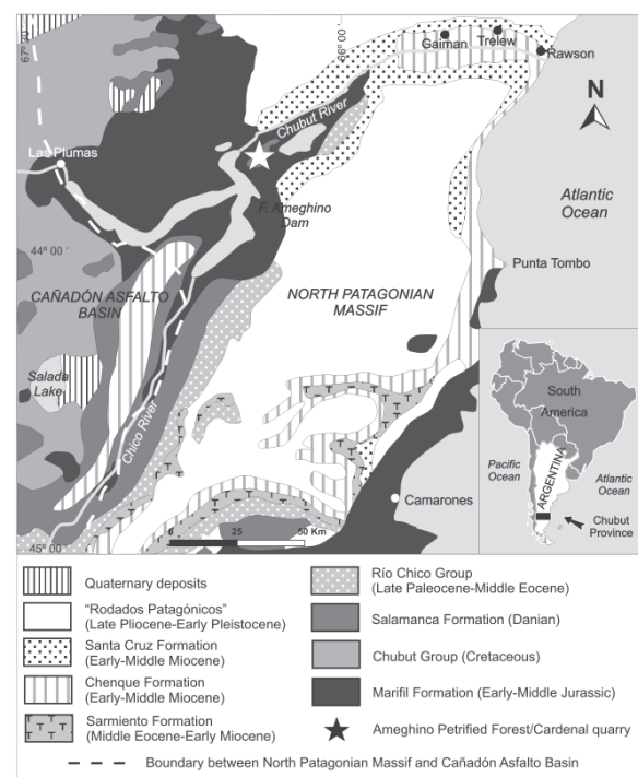
FIGURE 1 | Geological sketch of the study area (modified from Ardolivo et al., 2004) located in the northeast of Chubut province, neighbouring the Northpatagonian Massif (Hervé et al., 2008) and the Cañadón Asfalto Basin (Cortiñas, 1996). The star shows the location of the Ameghino Petrified Forest.
