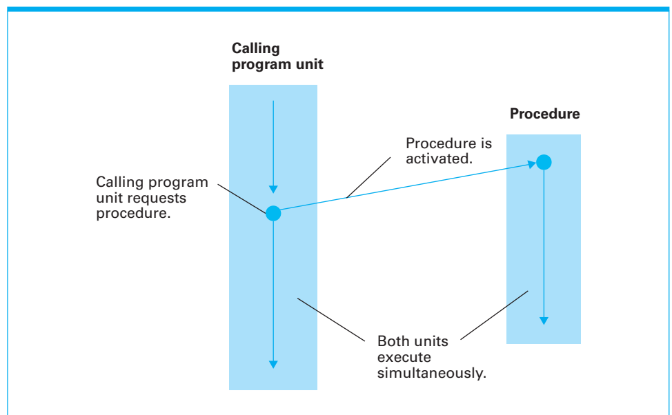
Figure 6.23 Spawning threads
