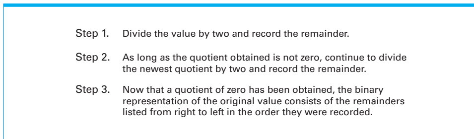
Figure 1.17 An algorithm for finding the binary representation of a positive integer
