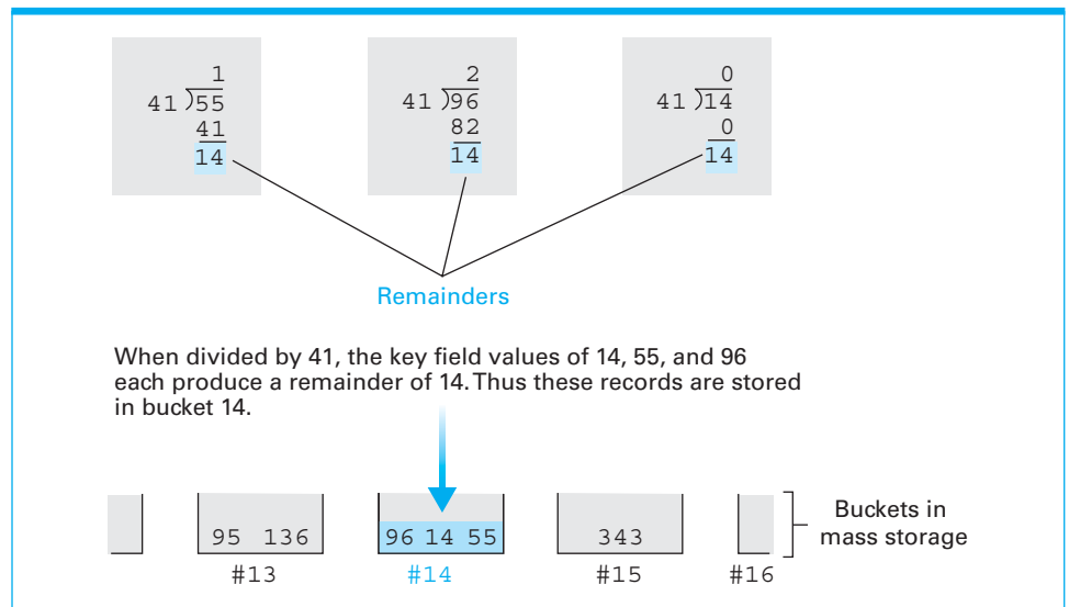
Figure 9.19 The rudiments of a hashing system
