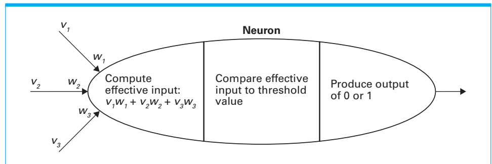
Figure 11.16 The activities within a neuron
