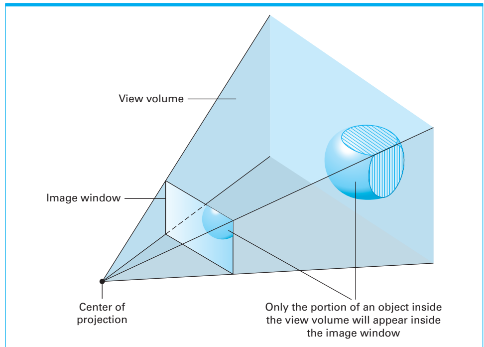
Figure 10.10 Identifying the region of the scene that lies inside the view volume
