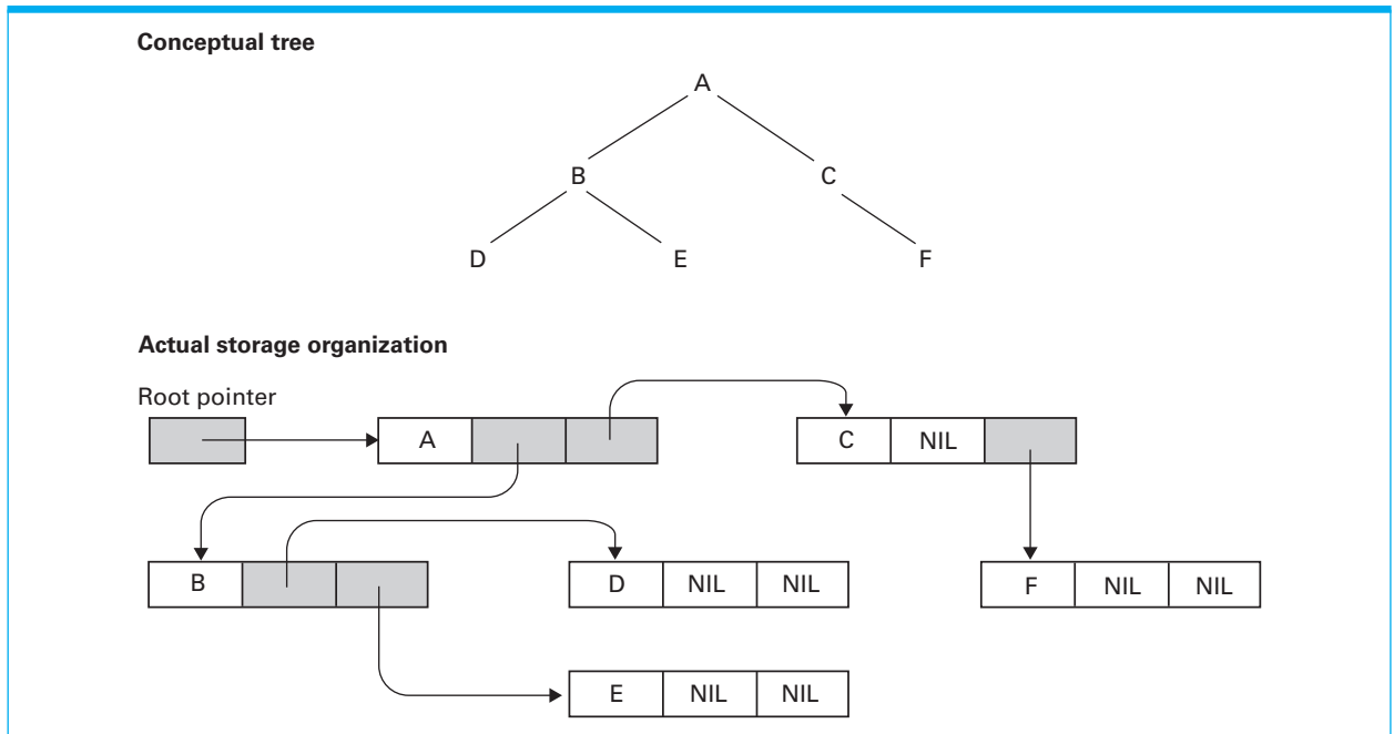
Figure 8.16 The conceptual and actual organization of a binary tree using a linked storage system
