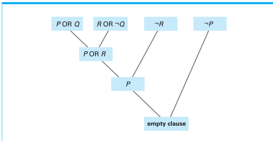
Figure 6.25 Resolving the statements (P \text{ OR } Q) , (R \text{ OR } \neg Q) , \neg R , and \neg P
