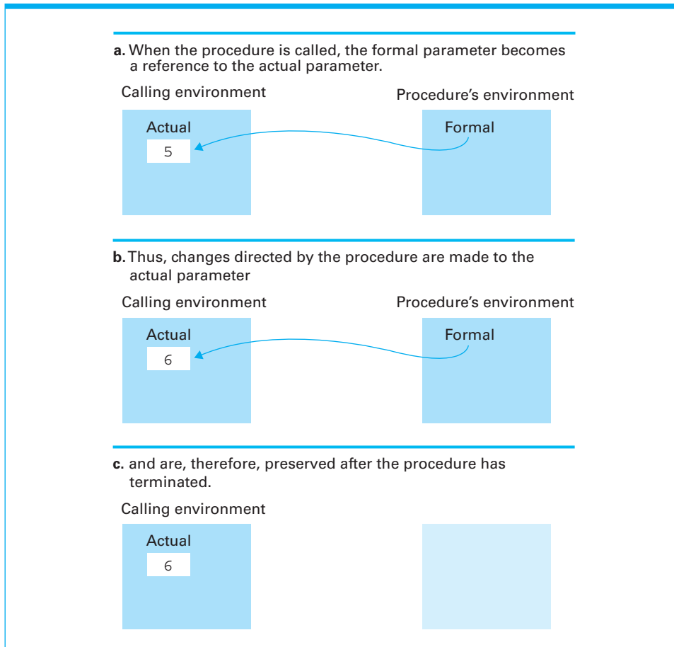
Figure 6.11 Executing the procedure Demo and passing parameters by reference
