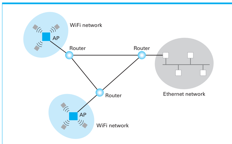
Figure 4.5 Routers connecting two WiFi networks and an Ethernet network to form an internet
