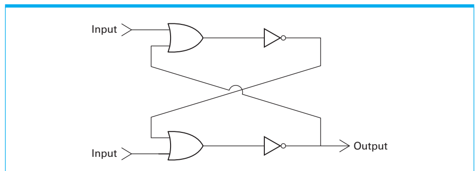
Figure 1.5 Another way of constructing a flip-flop
