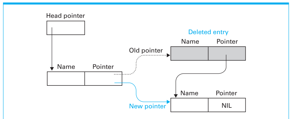
Figure 8.10 Deleting an entry from a linked list
