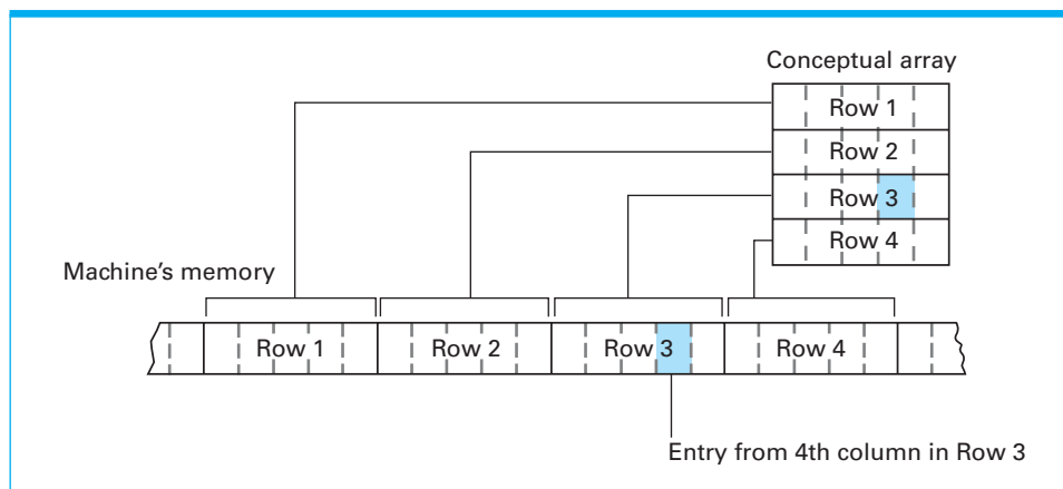
Figure 8.6 A two-dimensional array with four rows and five columns stored in row major order
