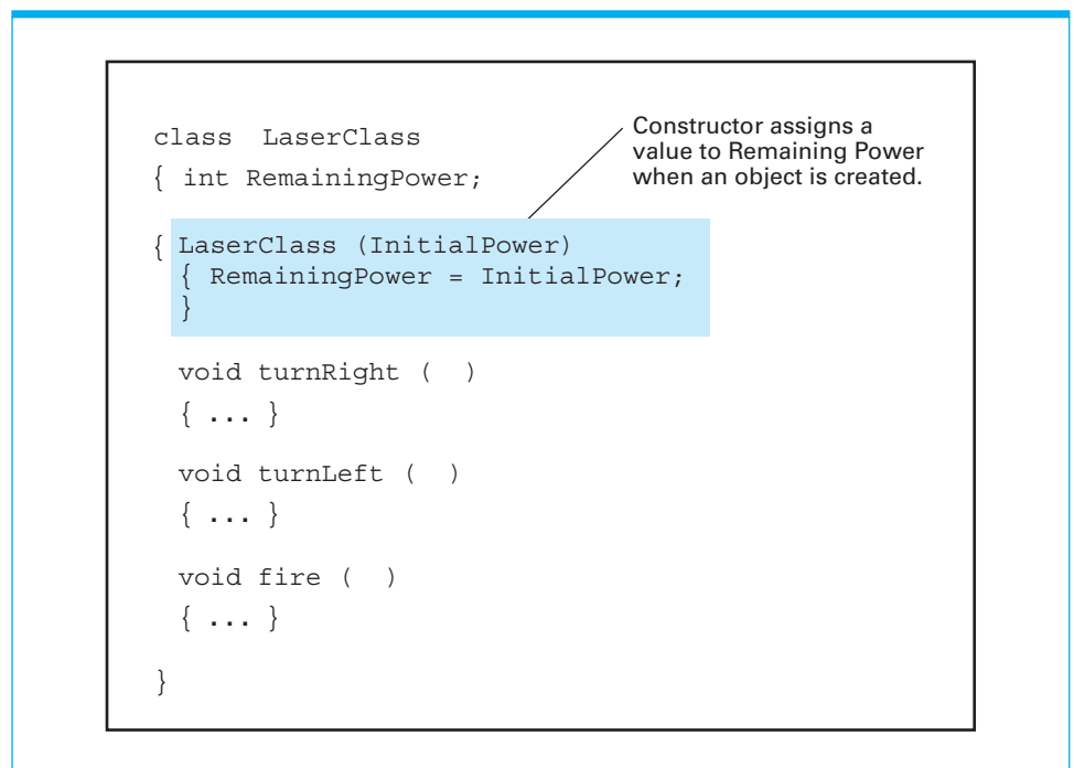
Figure 6.21 A class with a constructor
