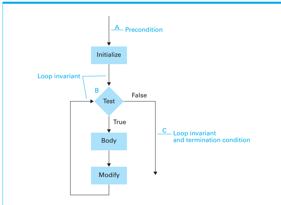
Figure 5.23 The assertions associated with a typical while structure
