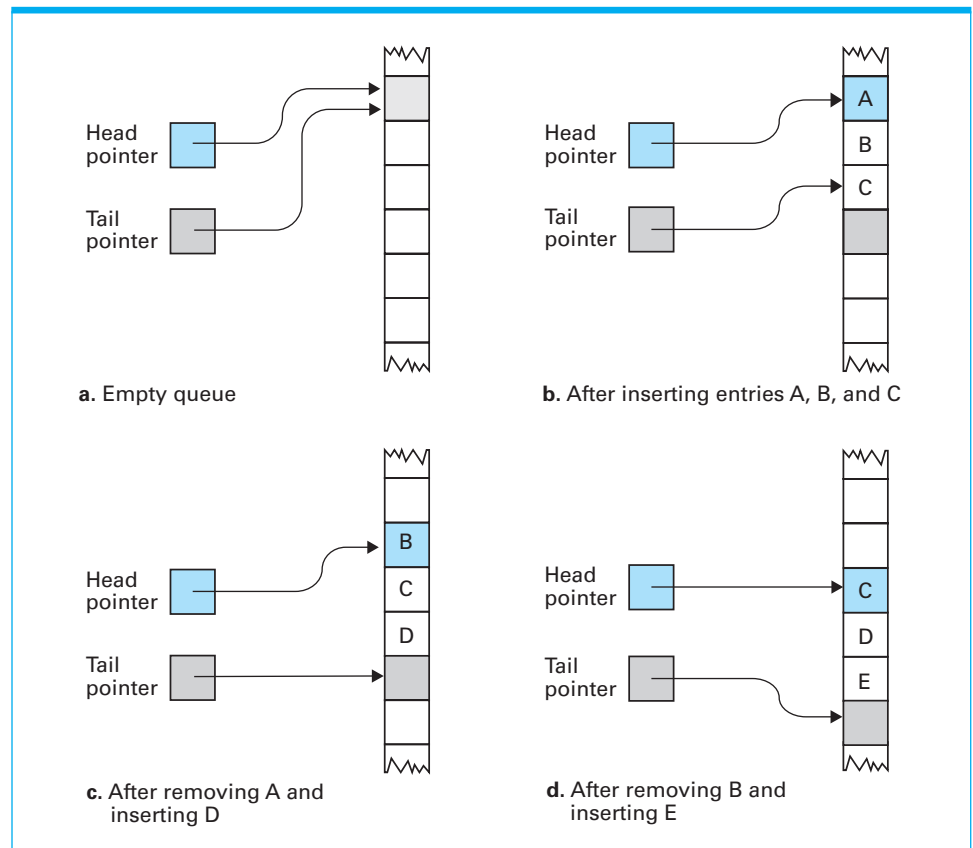
Figure 8.13 A queue implementation with head and tail pointers. Note how the queue crawls through memory as entries are inserted and removed.
