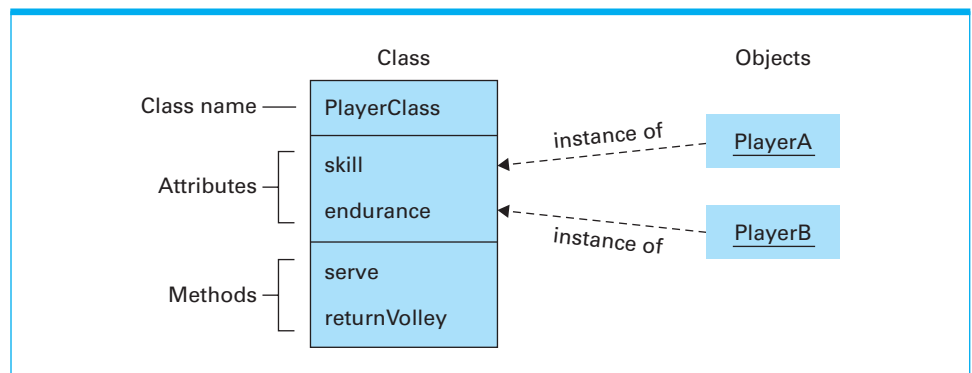
Figure 7.4 The structure of PlayerClass and its instances
