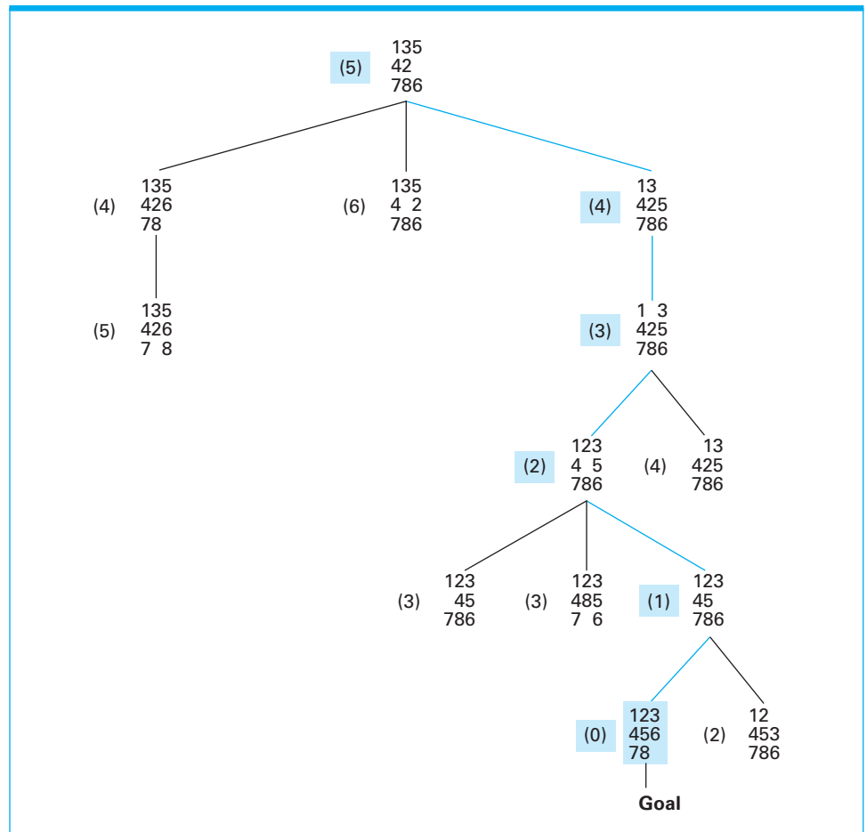
Figure 11.14 The complete search tree formed by our heuristic system
