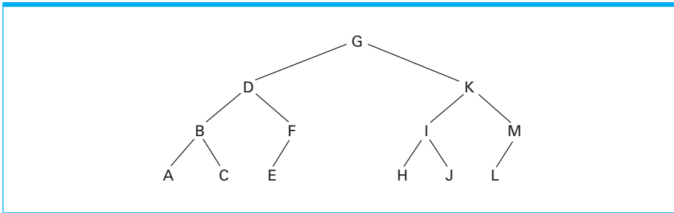
Figure 8.20 The letters A through M arranged in an ordered tree
