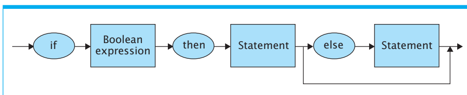
Figure 6.14 A syntax diagram of our if-then-else pseudocode statement
