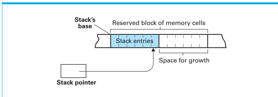
Figure 8.12 A stack in memory
