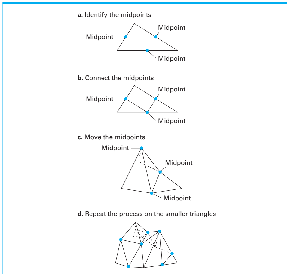
Figure 10.5 Growing a polygonal mesh for a mountain range
