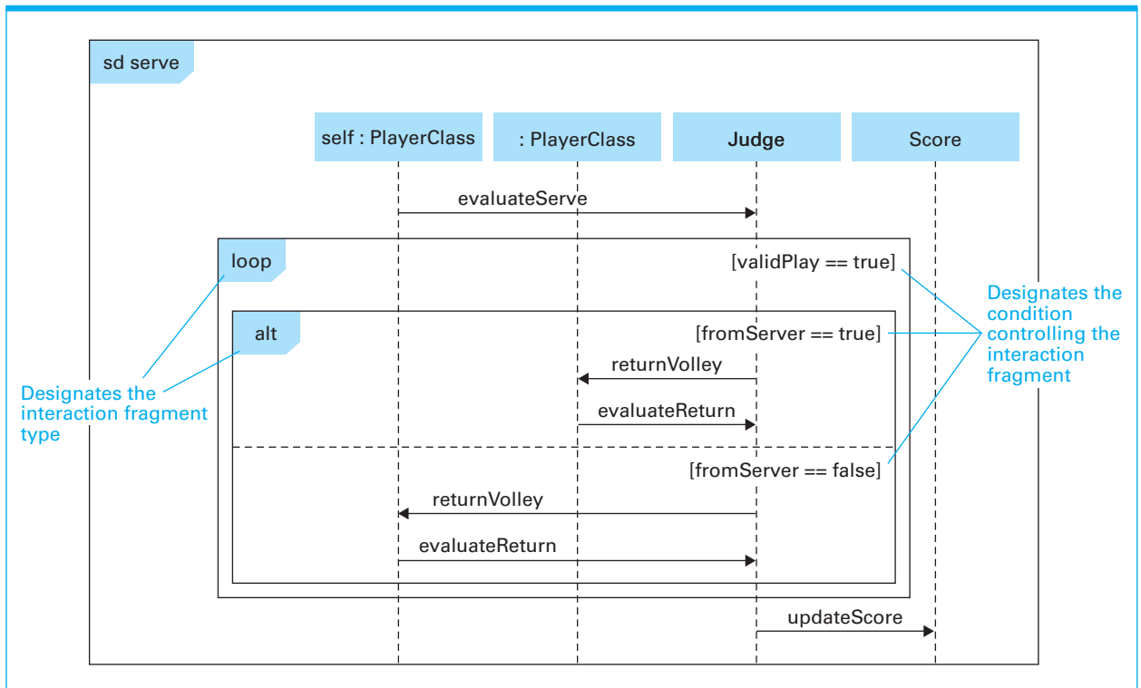
Figure 7.13 A sequence diagram depicting a generic volley
