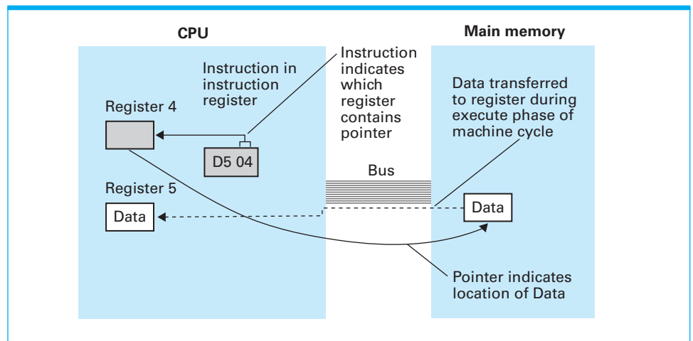
Figure 8.29 Loading a register from a memory cell that is located by means of a pointer stored in a register
