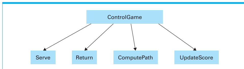
Figure 7.3 A simple structure chart
