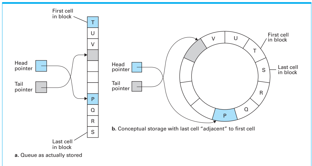
Figure 8.14 A circular queue containing the letters P through V
