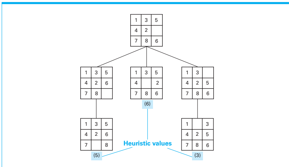
Figure 11.13 The search tree after three passes
