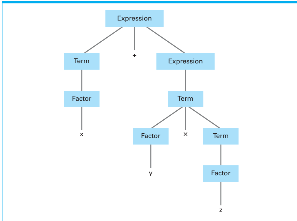
Figure 6.16 The parse tree for the string x + y + z based on the syntax diagrams in Figure 6.15
