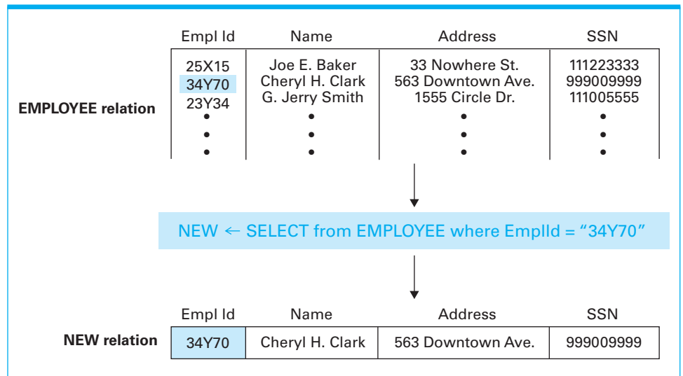
Figure 9.8 The SELECT operation
