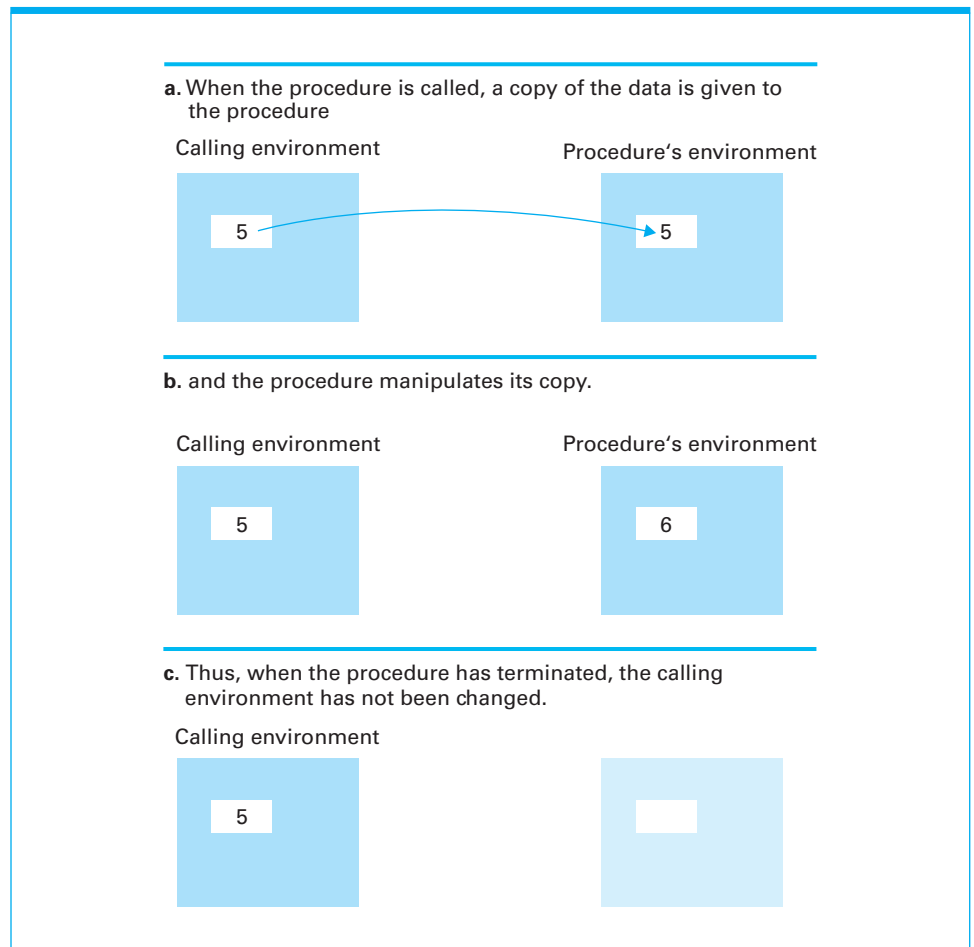
Figure 6.10 Executing the procedure Demo and passing parameters by value
