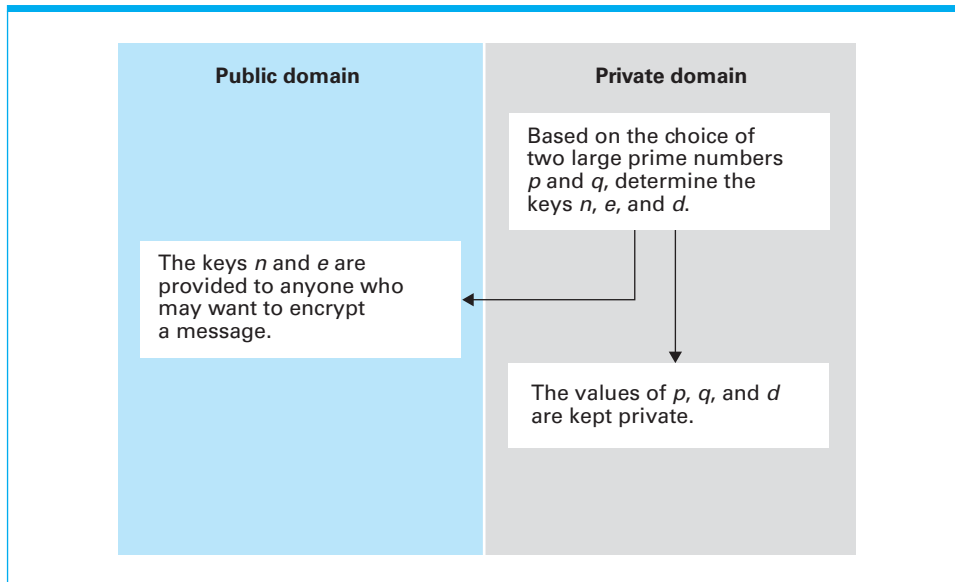
Figure 12.14 Establishing an RSA public key encryption system
