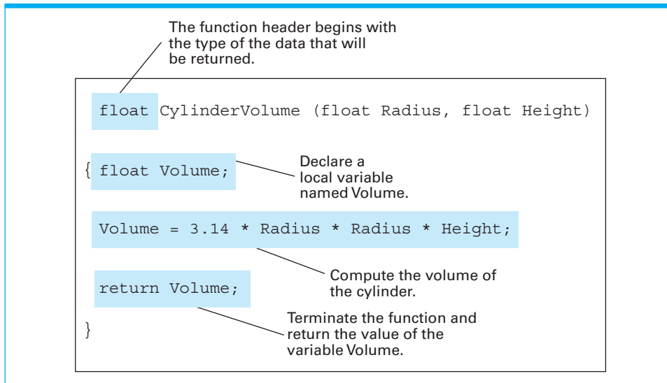
Figure 6.12 The function CylinderVolume written in the programming language C
