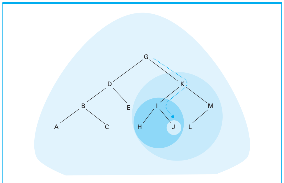
Figure 8.22 The successively smaller trees considered by the procedure in Figure 8.21 when searching for the letter J
