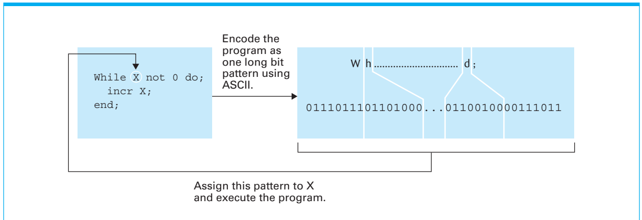
Figure 12.6 Testing a program for self-termination
