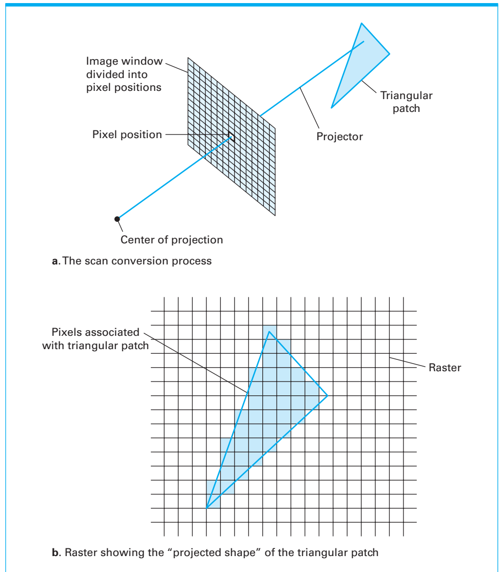
Figure 10.11 The scan conversion of a triangular patch
