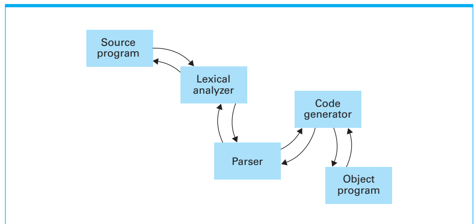
Figure 6.18 An object-oriented approach to the translation process
