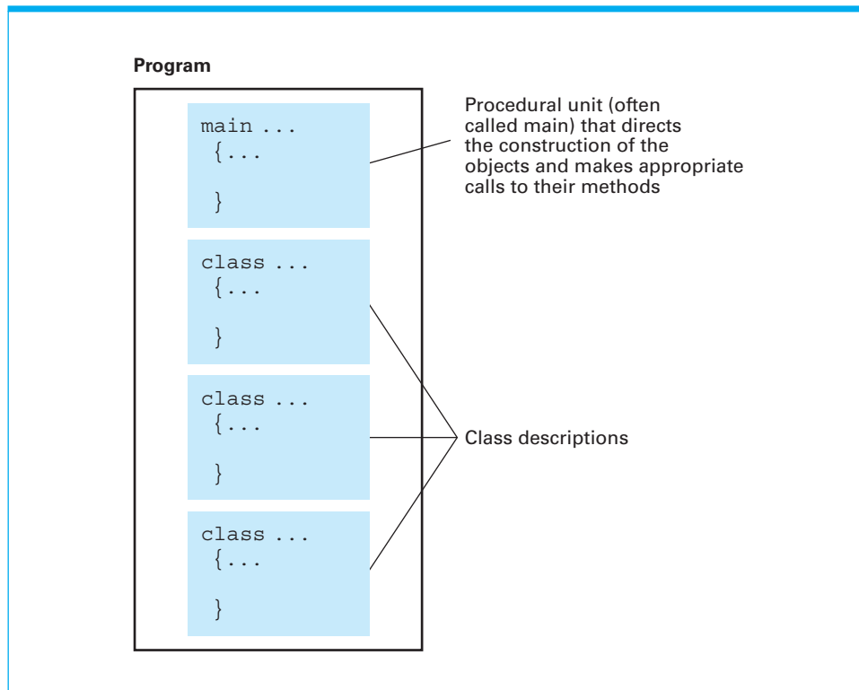
Figure 6.20 The structure of a typical object-oriented program
