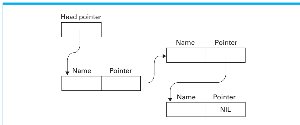
Figure 8.9 The structure of a linked list
