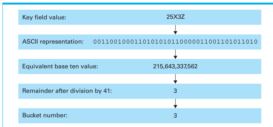
Figure 9.18 Hashing the key field value 25X3Z to one of 41 buckets
