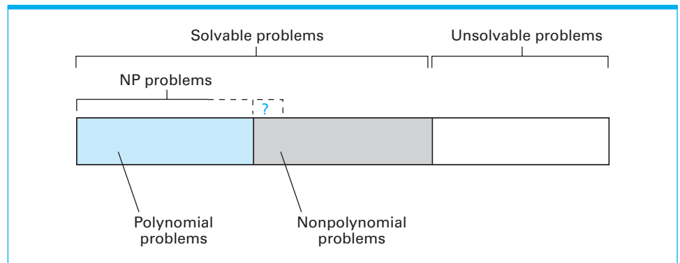
Figure 12.12 A graphic summation of the problem classification
