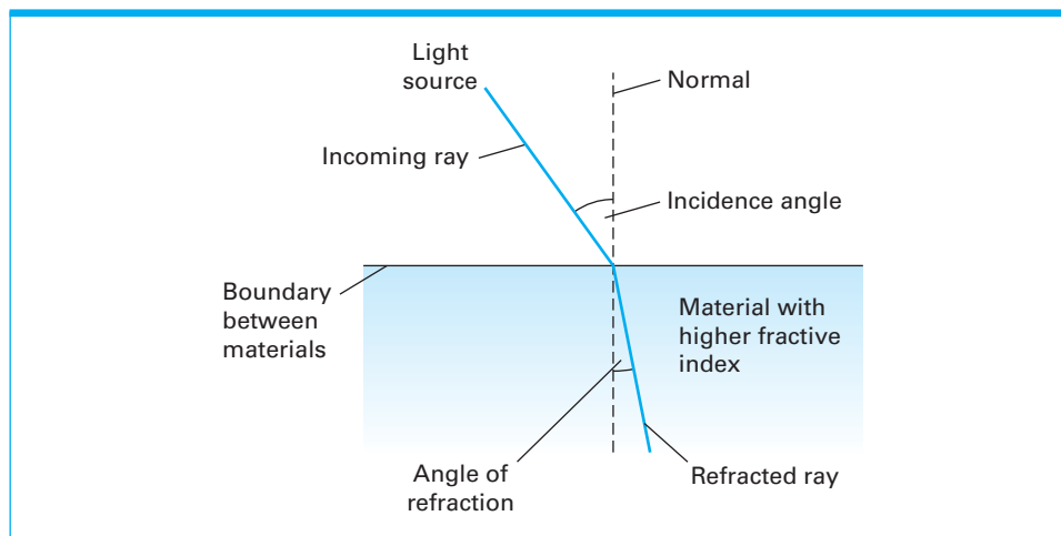
Figure 10.9 Refracted light
