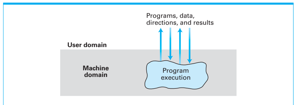
Figure 3.2 Interactive processing
