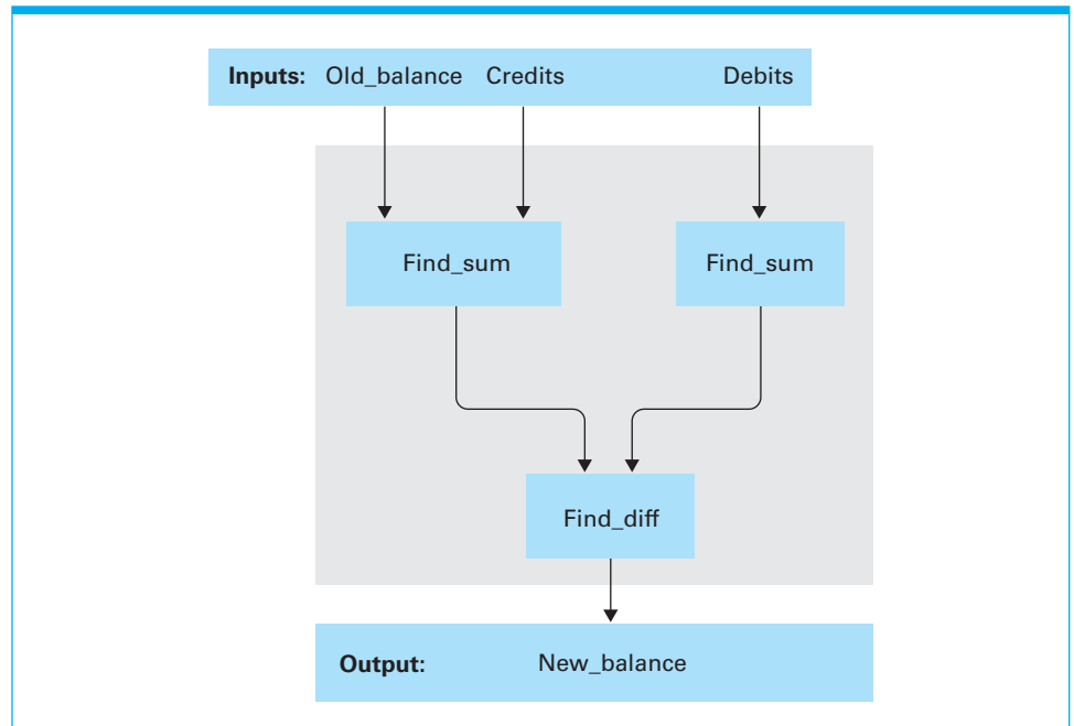
Figure 6.3 A function for checkbook balancing constructed from simpler functions
