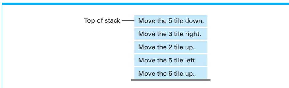
Figure 11.8 Productions stacked for later execution
