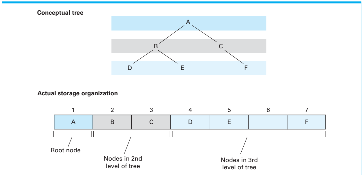
Figure 8.17 A tree stored without pointers
