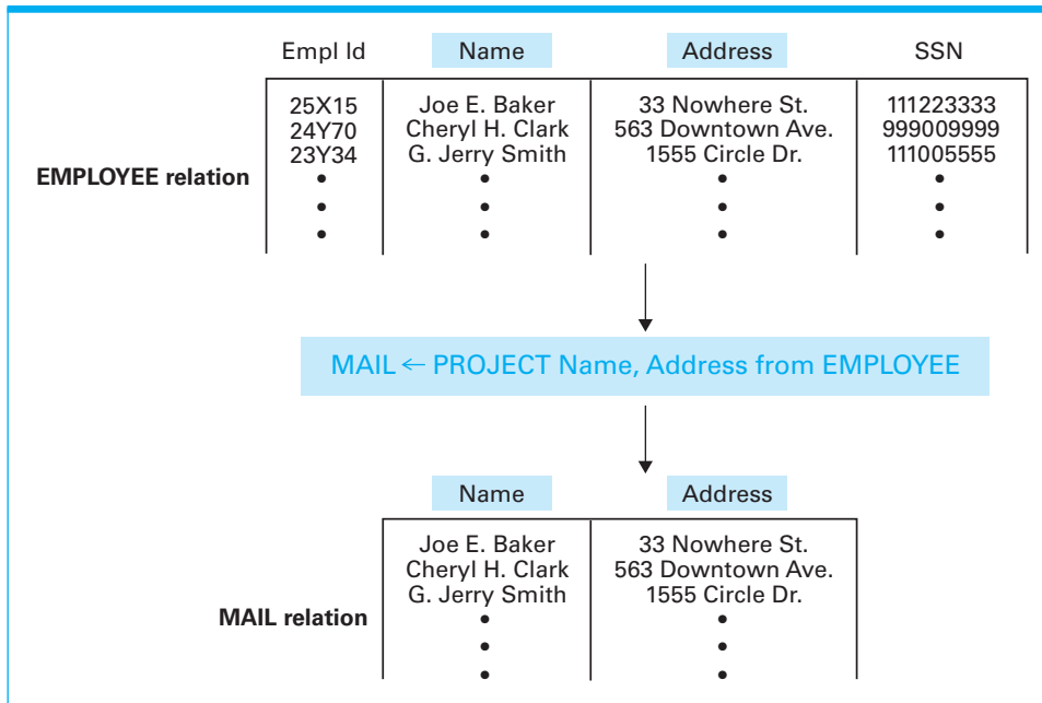
Figure 9.9 The PROJECT operation
