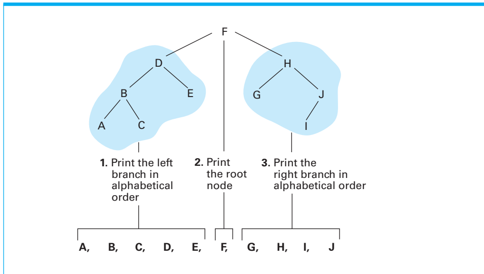
Figure 8.23 Printing a search tree in alphabetical order
