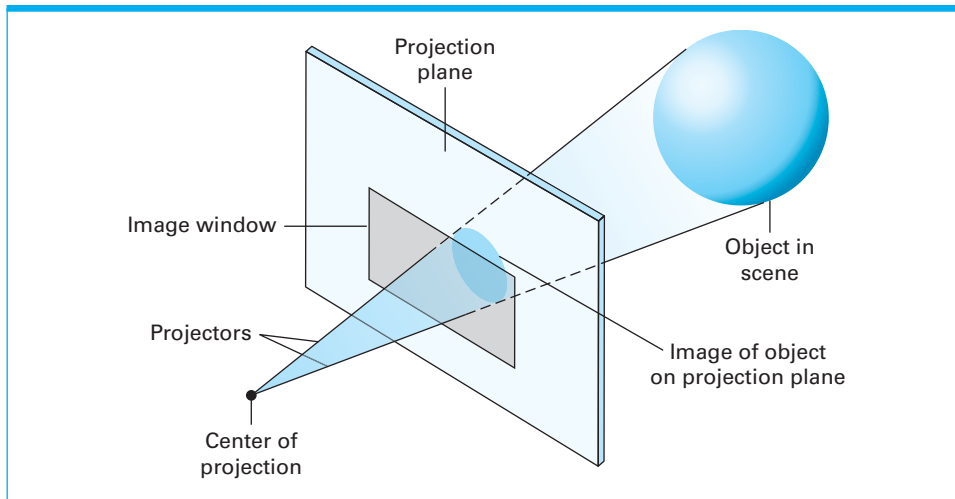
Figure 10.2 The 3D graphics paradigm
