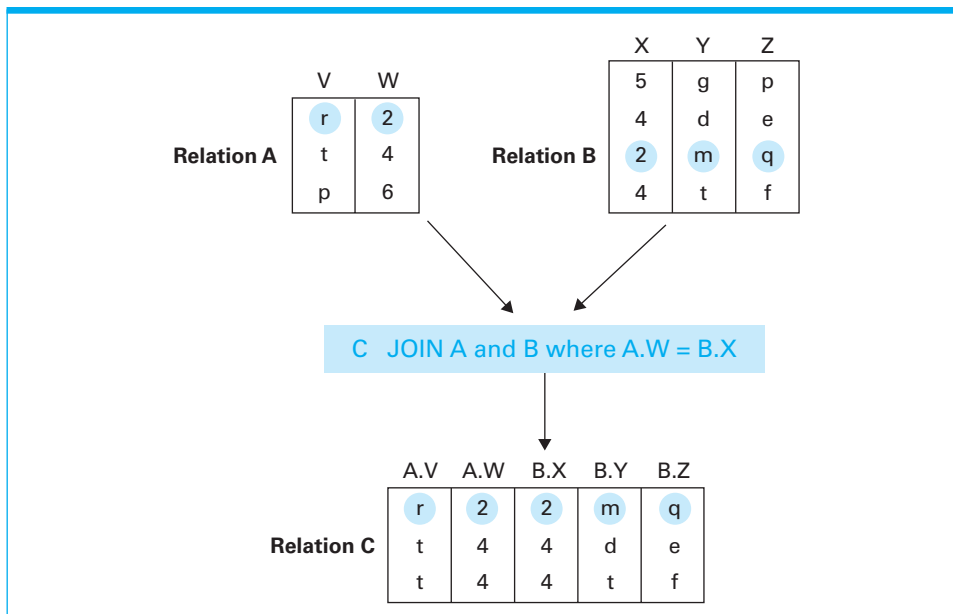
Figure 9.10 The JOIN operation
