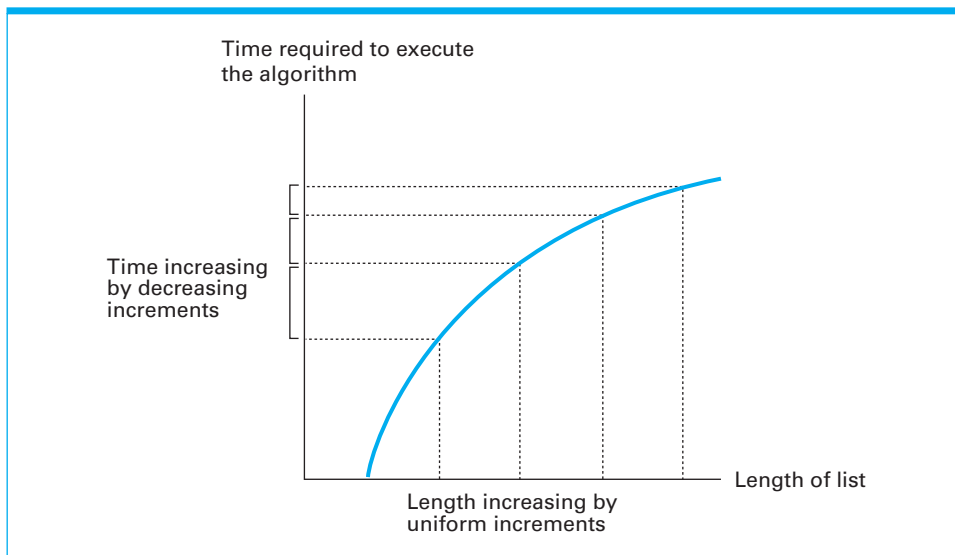
Figure 5.20 Graph of the worst-case analysis of the binary search algorithm
