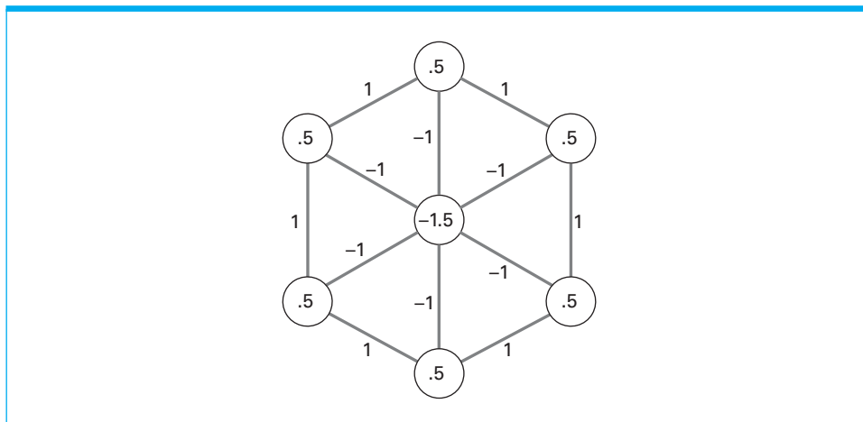
Figure 11.21 An artificial neural network implementing an associative memory
