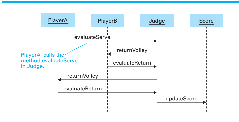
Figure 7.5 The interaction between objects resulting from PlayerA's serve
