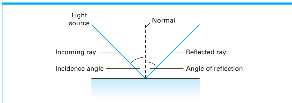
Figure 10.7 Reflected light
