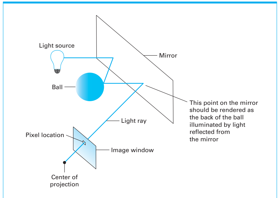
Figure 10.15 Ray tracing
