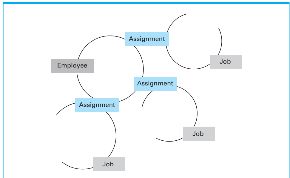
Figure 9.13 The associations between objects in an object-oriented database
