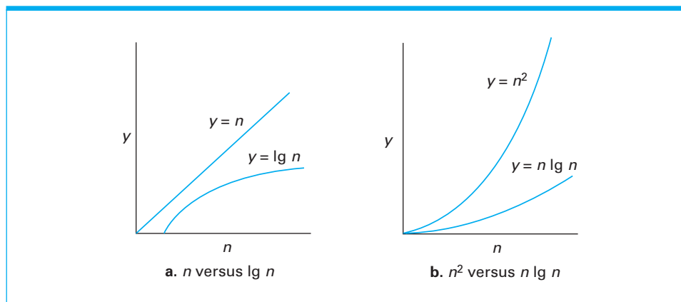
Figure 12.11 Graphs of the mathematical expressions n , \lg n , n \lg n , and n^2
