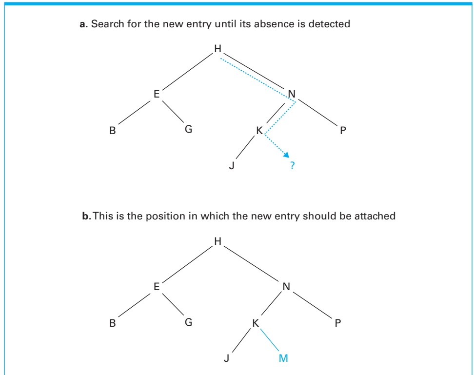
Figure 8.25 Inserting the entry M into the list B, E, G, H, J, K, N, P stored as a tree
