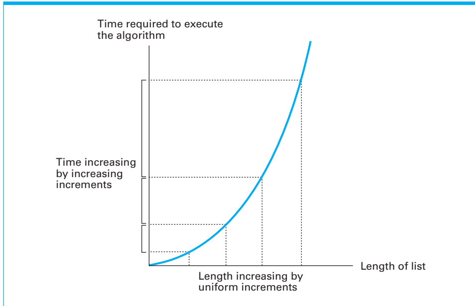
Figure 5.19 Graph of the worst-case analysis of the insertion sort algorithm
