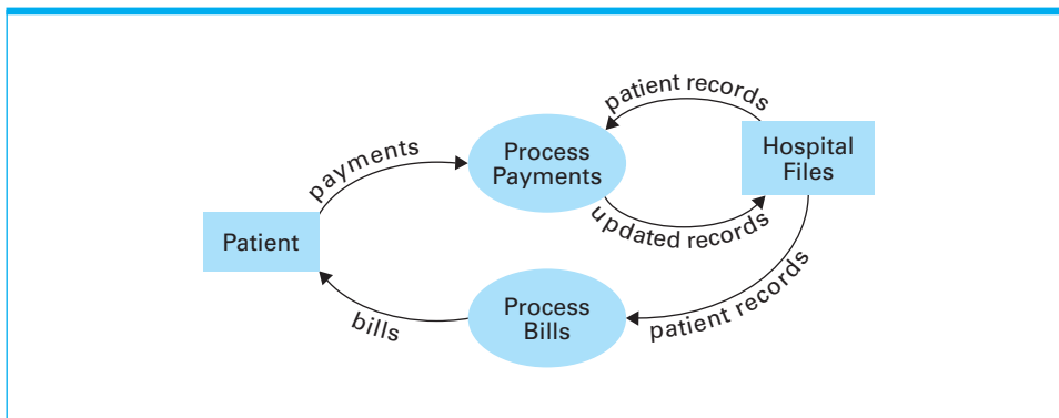
Figure 7.8 A simple dataflow diagram
