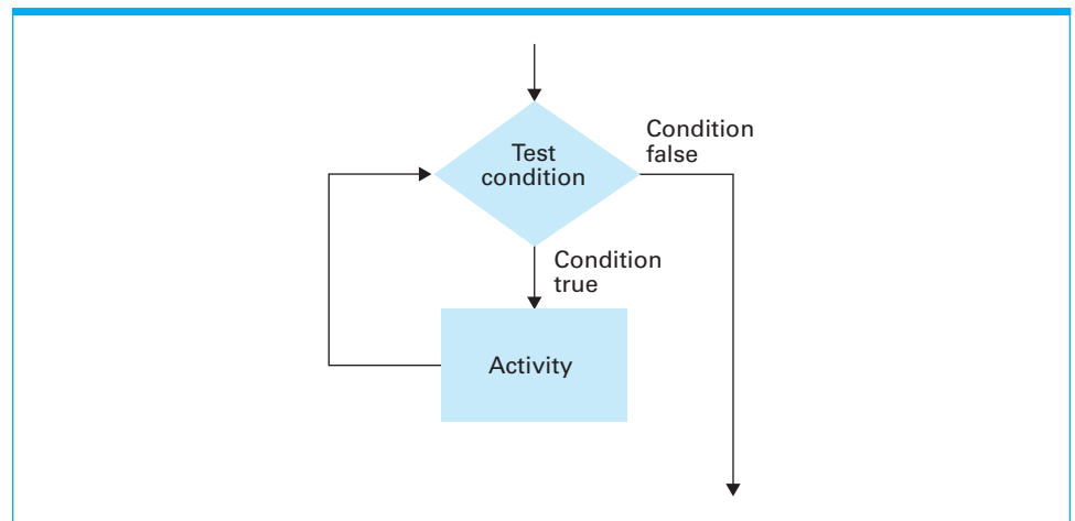
Figure 5.8 The while loop structure
