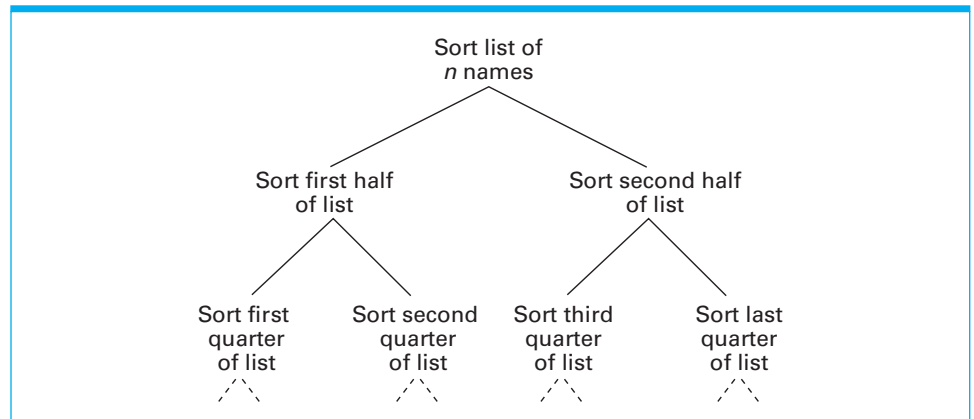
Figure 12.10 The hierarchy of problems generated by the merge sort algorithm
