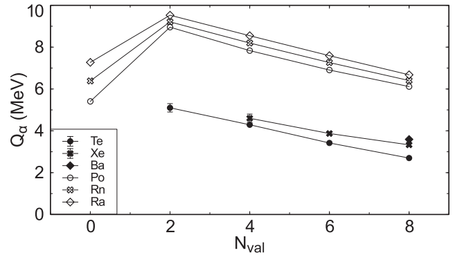
FIG. 4. Q_\alpha values of the even-even \alpha emitters in the ^{100}\text{Sn} region (solid symbols) and in the ^{208}\text{Pb} region (open symbols) as a function of the number of valence neutrons.
