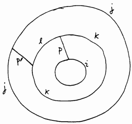
graphical formulas for the b monodromy
