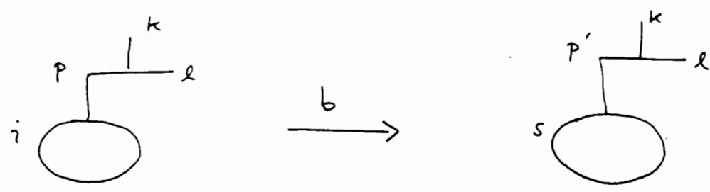
the general b monodromy
