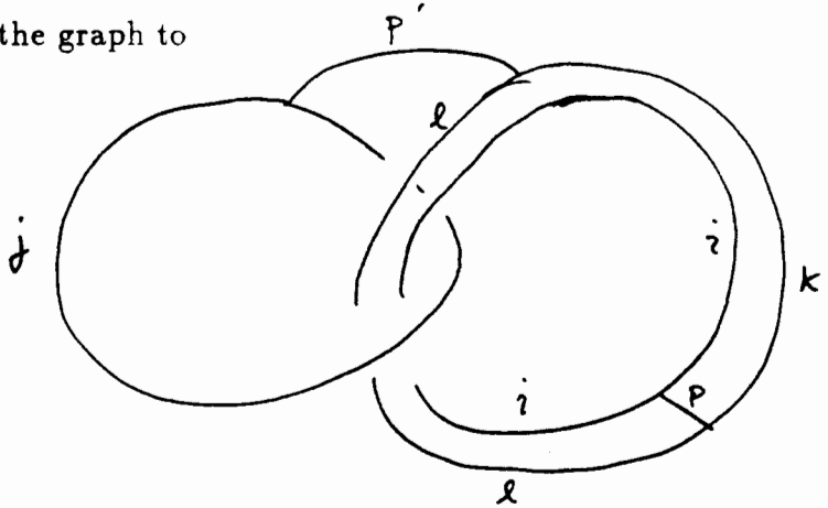
A deformation of the same graph
