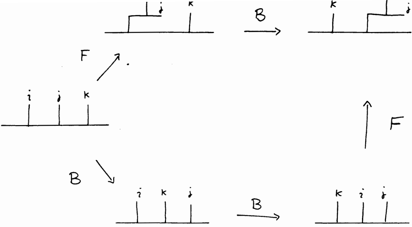
pentagon of dual diagrams
