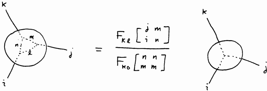
another link in a three ball
