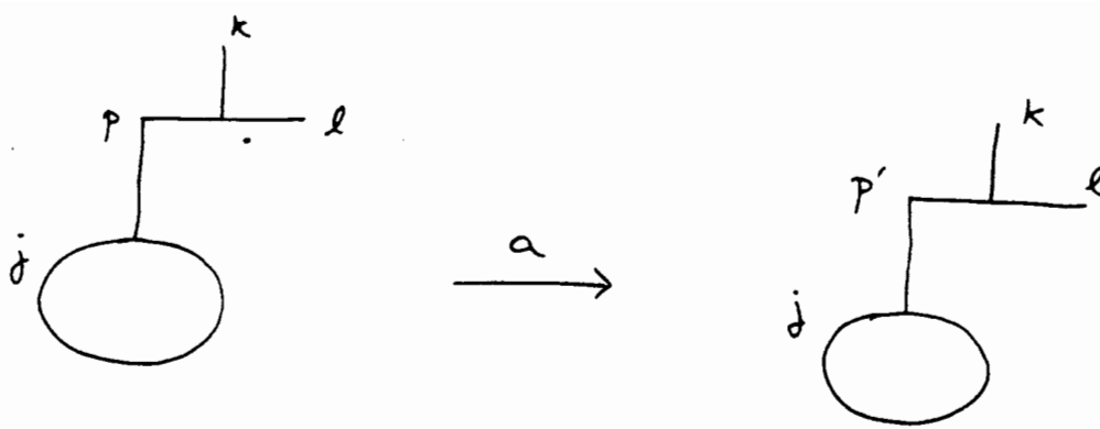
the general a monodromy
