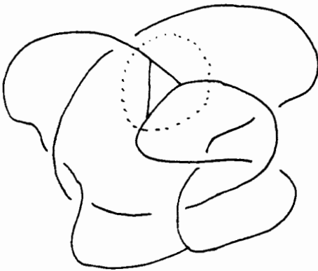
a complicated link
