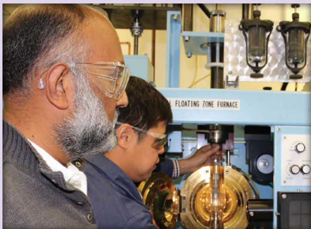
Easo George and Hongbin Bei with the ORNL high-temperature optical floating zone furnace used to produce monocrystalline molybdenum alloy micropillars.
