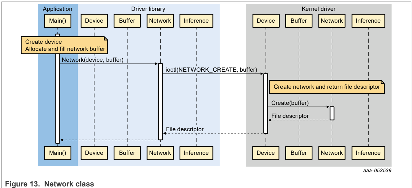
Figure 13. Network class
