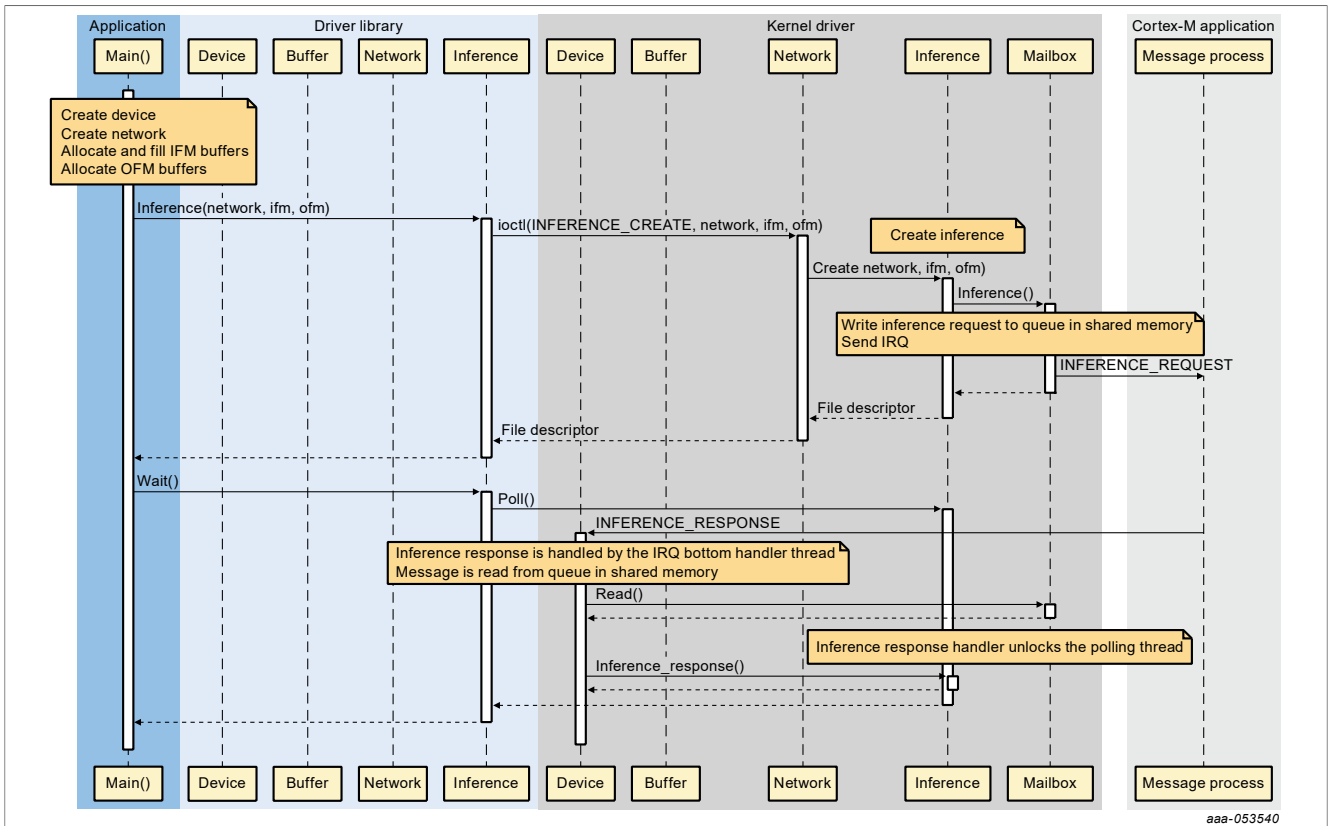
Figure 14. Inference class
