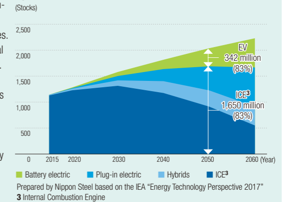
Global technology penetrations in LDV stock by 2DS scenario
