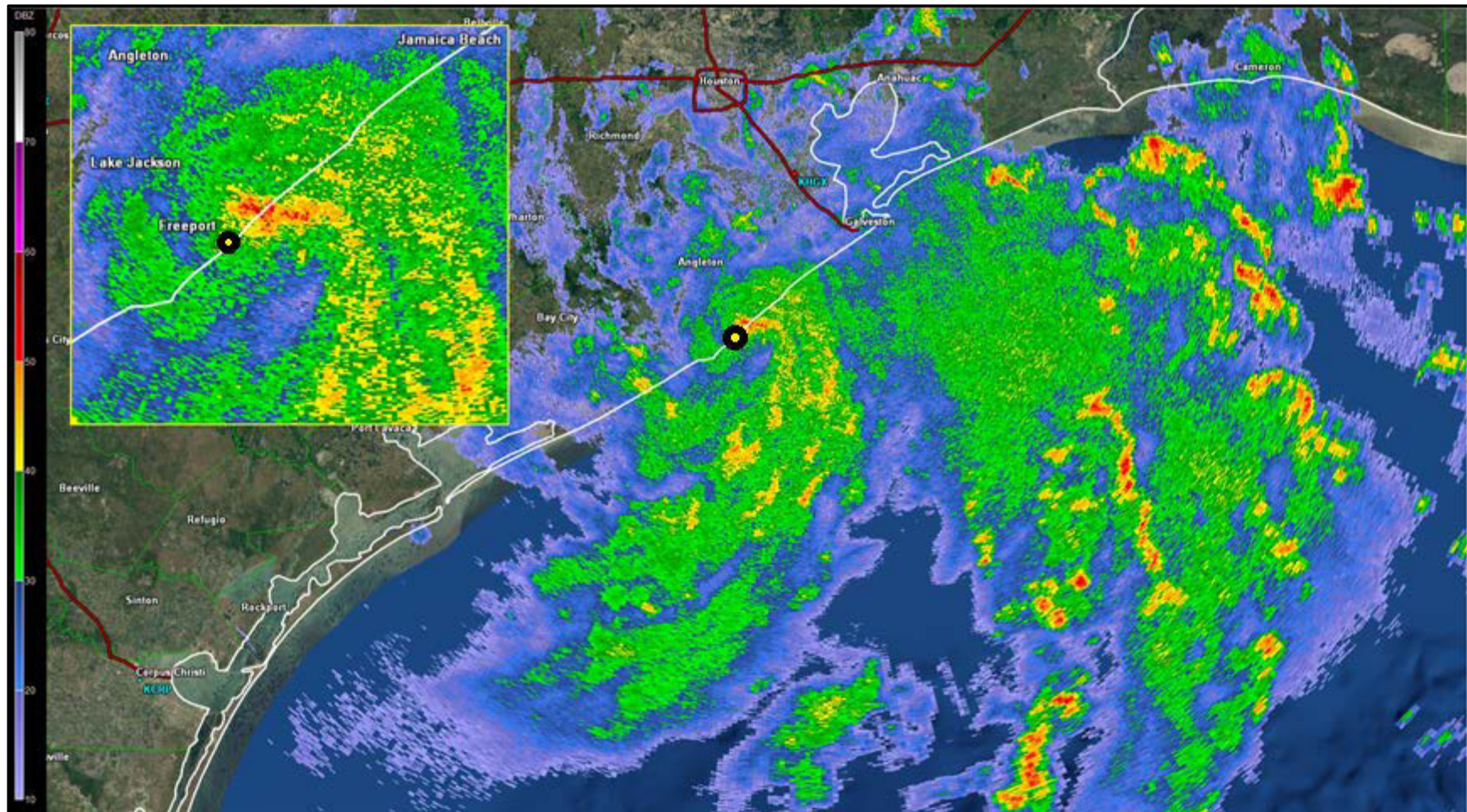
Figure 1. KHXG WSR-88D radar reflectivity (dBZ; 0.5° elev. angle) at 1743 UTC 17 September, very close to the landfall time of Imelda along the Texas coast near Freeport. Center location indicated by yellow dot on inset and larger image. Graphic courtesy of GR2Analyst, Gibson Ridge Software, LLC, Suwanee, Georgia.
