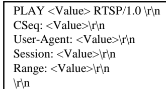
Fig. 3. Grammar for the RTSP PLAY client request.
