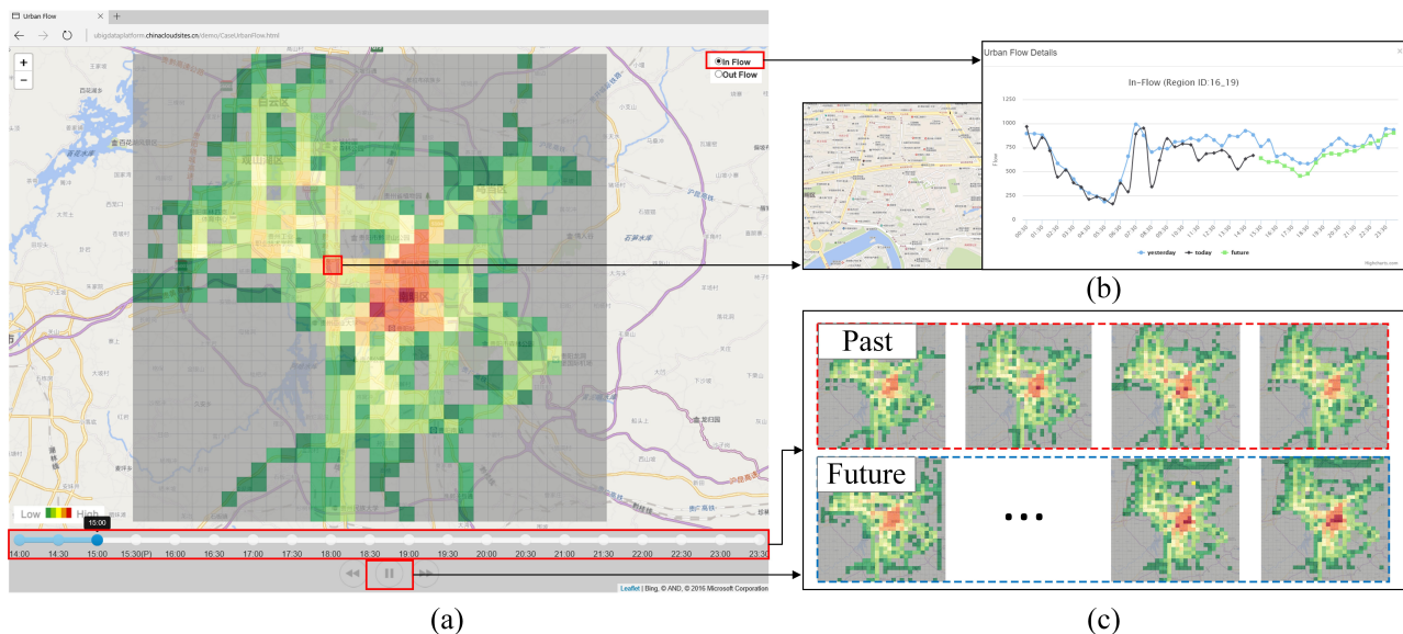
Figure 2: UrbanFlow: A real-time crowd flow forecasting system
