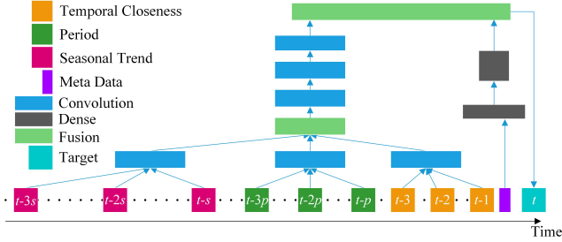
Figure 3: DeepST Architecture.
