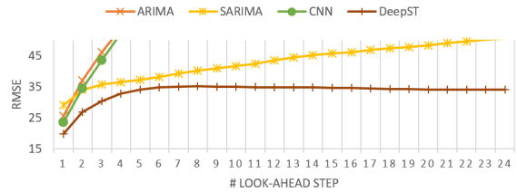
Figure 6: Multi-step Ahead Prediction
