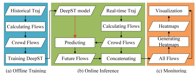
Figure 1: System Framework. Traj: trajectories.
