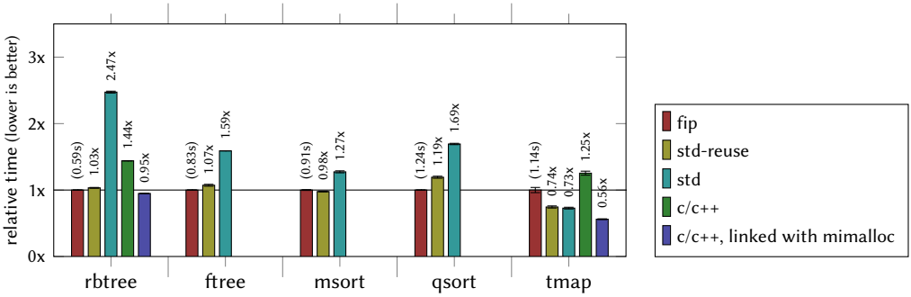
Fig. 11. Benchmarks on Ubuntu 22.04.2 (AMD 7950x), Koka v2.4.1-dev-fbip.
