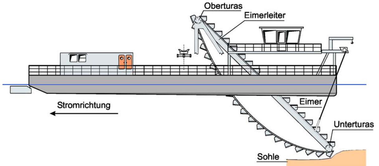
14-3 Eimerketten-Nassbagger
