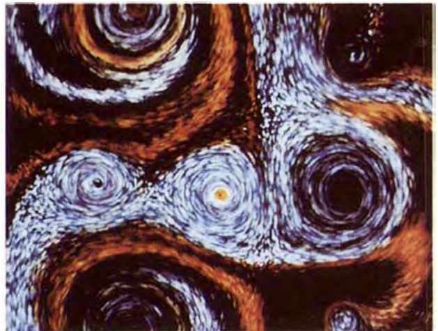
Figure 5: (a) Burning Letters, (b) Vortex Field.
