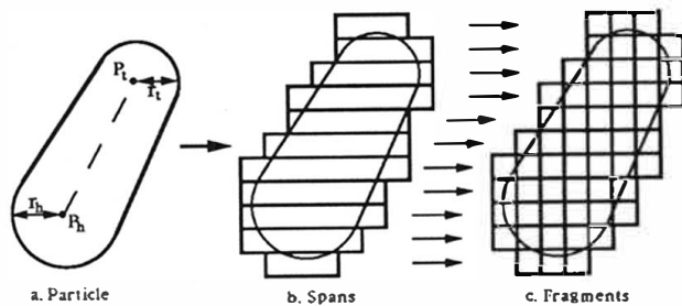
Figure 3: Particle Dicing.
