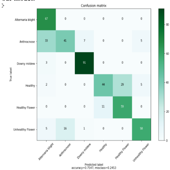
Fig.10. Confusion Matrix
