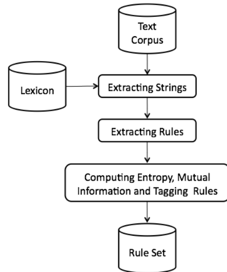
Figure 1: Rule Training.
