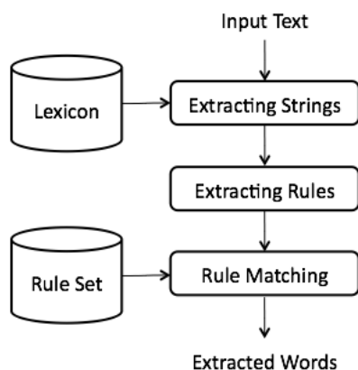
Figure 2: Word Extraction.
