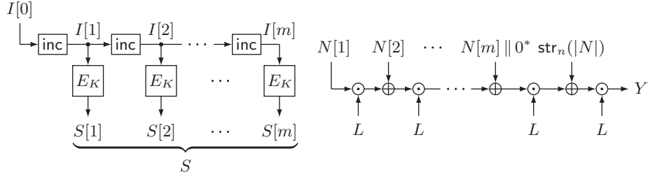
Fig. 3. Overall structure of (C, T) \leftarrow \text{GCM-}\mathcal{E}_K^{N,A}(M)
