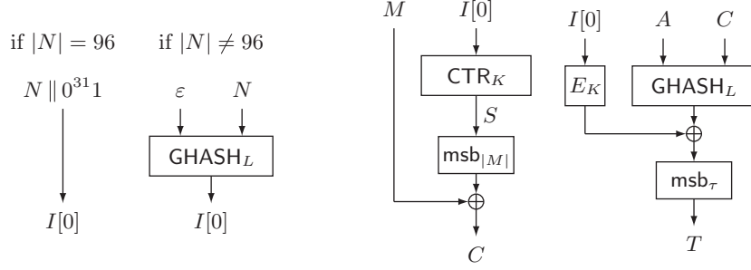
Fig. 3. Overall structure of (C, T) \leftarrow \text{GCM-}\mathcal{E}_K^{N,A}(M)
