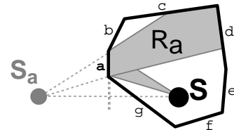
Figure 5: Beam tracing culls invisible virtual sources.
