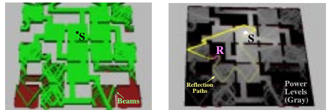
Figure 18: Eighth-order specular reflection beams (left) and predicted power levels (right) in Maze model.
