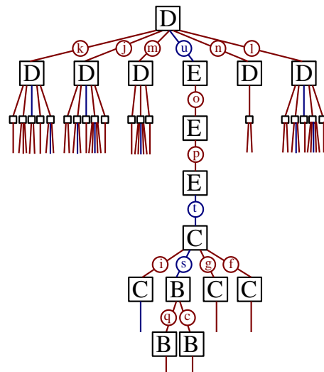
Figure 10: Beam tree.
