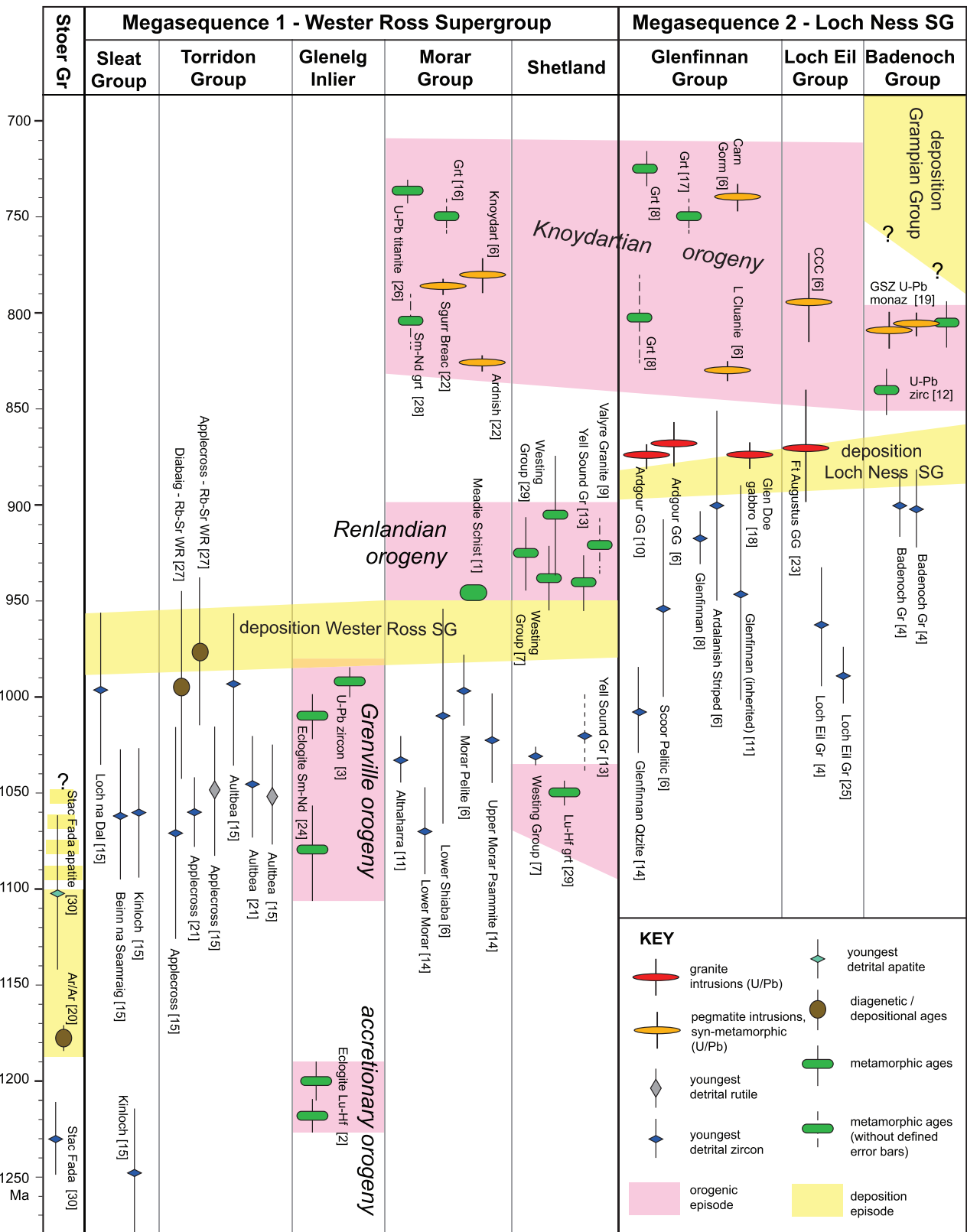
Fig. 4.4. Overview of radiometric age constraints in Northern Scotland, provided by youngest detrital zircon and rutile ages, metamorphic and intrusive ages, and depositional/diagenetic ages. CCC, Cruachan Coille a'Chait; GSZ, Grampian Shear Zone. Source: data after [1] and [2] Bird et al. (2018, 2023); [3] Brewer et al. (2003); [4], [5] and [6] Cawood et al. (2003, 2004, 2015); [7], [8] and [9] Cutts et al. (2009b, 2010, 2011); [10] and [11] Friend et al. (1997, 2003); [12] Highton et al. (1999); [13] Jahn et al. (2017); [14] Kirkland et al. (2008b); [15] Krabbendam et al. (2017a); [16] Mako et al. (2021); [17] Mazza et al. (2018); [18] Millar (1999); [19] Noble et al. (1996); [20] Parnell et al. (2011); [21] Rainbird et al. (2001); [22] and [23] Rogers et al. (1998, 2001); [24] Sanders et al. 1984; [25] Spencer et al. (2015); [26] Tanner and Evans (2003); [27] Turnbull et al. (1996); [28] Vance et al. (1998); [29] Walker et al. (2021); [30] Kenny et al. (2019). Modified after Krabbendam et al. (2022), BGS © UKRI.
