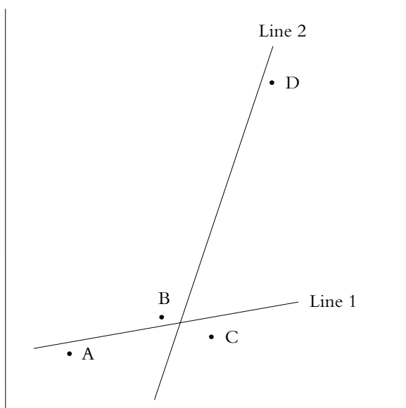
Figure 8. Least-Squares Regression
