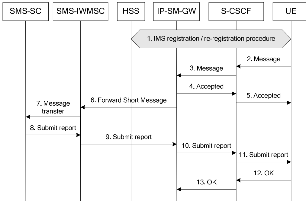
Figure 6.3: Successful encapsulated Short Message origination procedure
