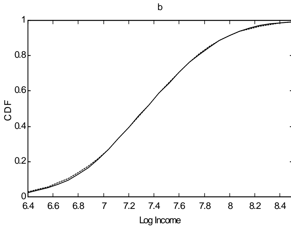
Figure 3: Simulated Group 1 (dashed) and Group 2 (solid) NCDS CDF's compared. a) Group 1 CDF plotted with Group 2 CDF. b) Group 1 CDF adjusted with MLE estimated a plotted with Group 2 CDF.
