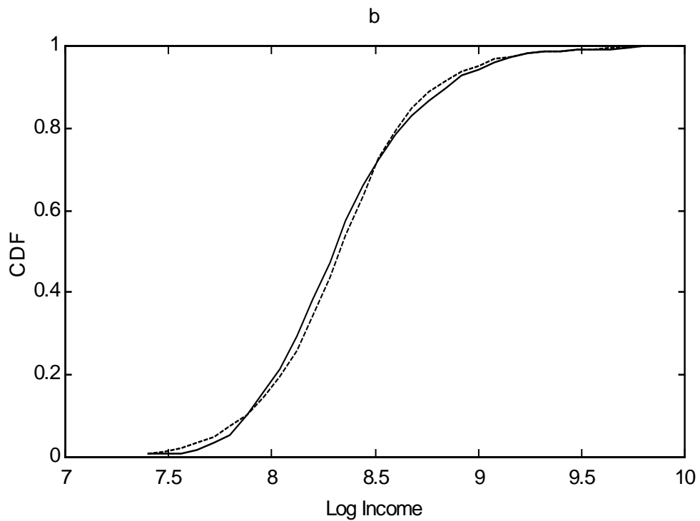
Figure 1: Group 1 (dashed) and Group 2 (solid) FES data compared. a) Group 1 CDF plotted with Group 2 CDF. b) Group 1 CDF adjusted with MLE estimated a plotted with Group 2 CDF.
