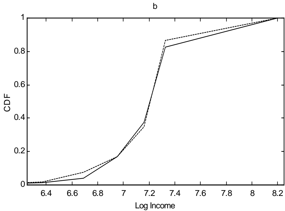
Figure 2: Group 1 (dashed) and Group 2 (solid) NCDS data compared. a) Group 1 CDF plotted with Group 2 CDF. b) Group 1 CDF adjusted with MLE estimated a plotted with Group 2 CDF.
