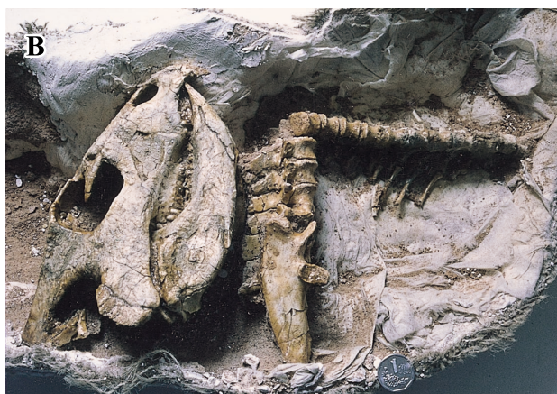
FIGURE 1. A. Phylogenetic relationships within the Neoceratopsian dinosaurs (Dong and Azuma, 1997); B. Archaeoceratops oshimai .
