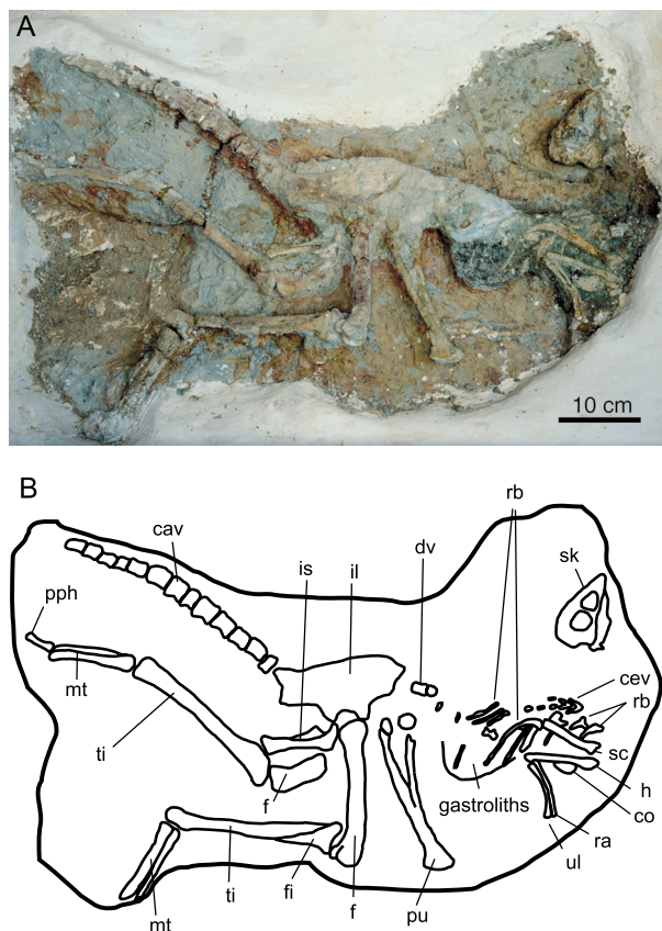
FIGURE 7. One of the small theropods collected at Suhongto, Alxa Gobi, Inner Mongolia. A juvenile ornithomimid: photograph (A) and line drawing (B). Abbreviations: cav , caudal vertebra; cev , cervical vertebra; co , coracoid; dv , dorsal vertebra; f , femur; fi , fibula; h , humerus; il , ilium; is , ischium; mt , metatarsal; pph , pedal phalanx; pu , pubis; ra , radius; rb , dorsal rib; sc , scapula; sk , skull; ti , tibia; ul , ulna.
