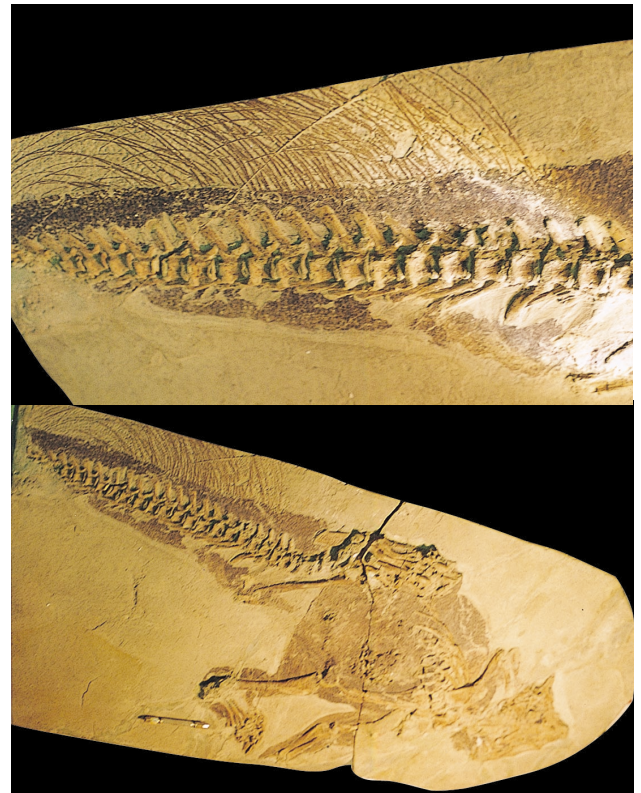
FIGURE 13. A skeleton of Psittacosaurus (horned dinosaur) with extraordinarily preserved integument.
