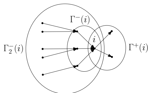
Figure 15.6: An illustration of the notation \Gamma^-(i) , \Gamma_2^-(i) , and \Gamma^+(i) .
