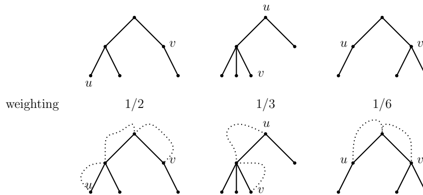
Figure 15.2: Two different ways of specifying a routing. On top is a weighted collection of trees. To route demand from u to v , we send 1/2 the demand along the u-v path in the first tree, 1/3 along the u-v path in the second tree, and a 1/6 in the last tree. On the bottom is a weighted collection of trees in which each tree edge has an associated path (shown as a dotted line only for edges on the u-v path). To route demand from u to v , we send flow along the concatenation of the paths associated with each in the u-v path in the tree; we send 1/2 the demand along the concatenation of the paths in the first tree, 1/3 along the concatenation of paths in the second tree, and 1/6 along the concatenation of paths in the last tree.
