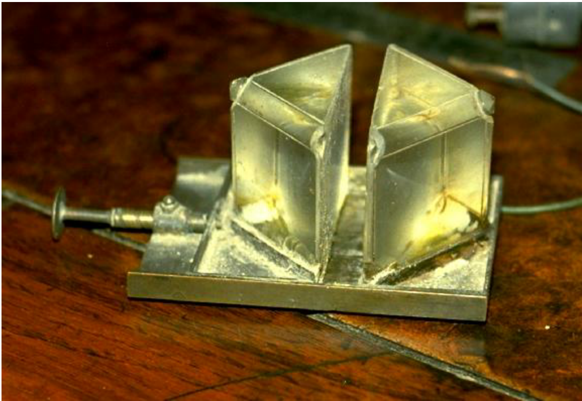
Figure 14. One of Bose's original double-prism attenuators, with adjustable air gap.
