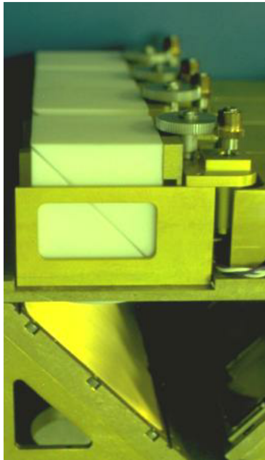
Figure 15. Four of the 8 double-prism attenuators used to control local oscillator injection into the NRAO 1.3-mm 8-beam receiver in use at the 12 Meter Telescope at Kitt Peak.
