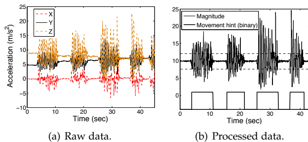
Fig. 5: Movement detection accuracy.
