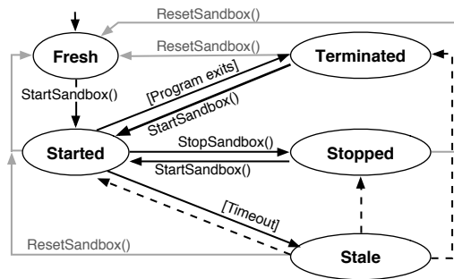
Fig. 2: The sandbox state machine maintained by the resource manager. StartSandbox, StopSandbox, and ResetSandbox are resource manager calls. [Program exits] and [Timeout] are sandbox events. Dashed arrows indicate an implicit event in which the sandbox recovers after a timeout.
