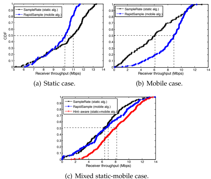
Fig. 6: Protocol throughput in three different scenarios.
