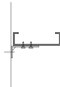
PLAN VIEW
