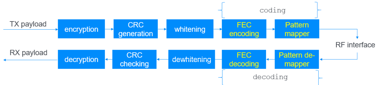
Figure 5 - FEC bit stream processing introduced in Bluetooth Core Specification Version 5.0
