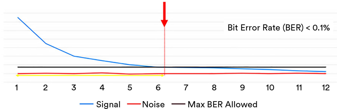
Figure 4 - Relationship between SNR and BER - not to scale
