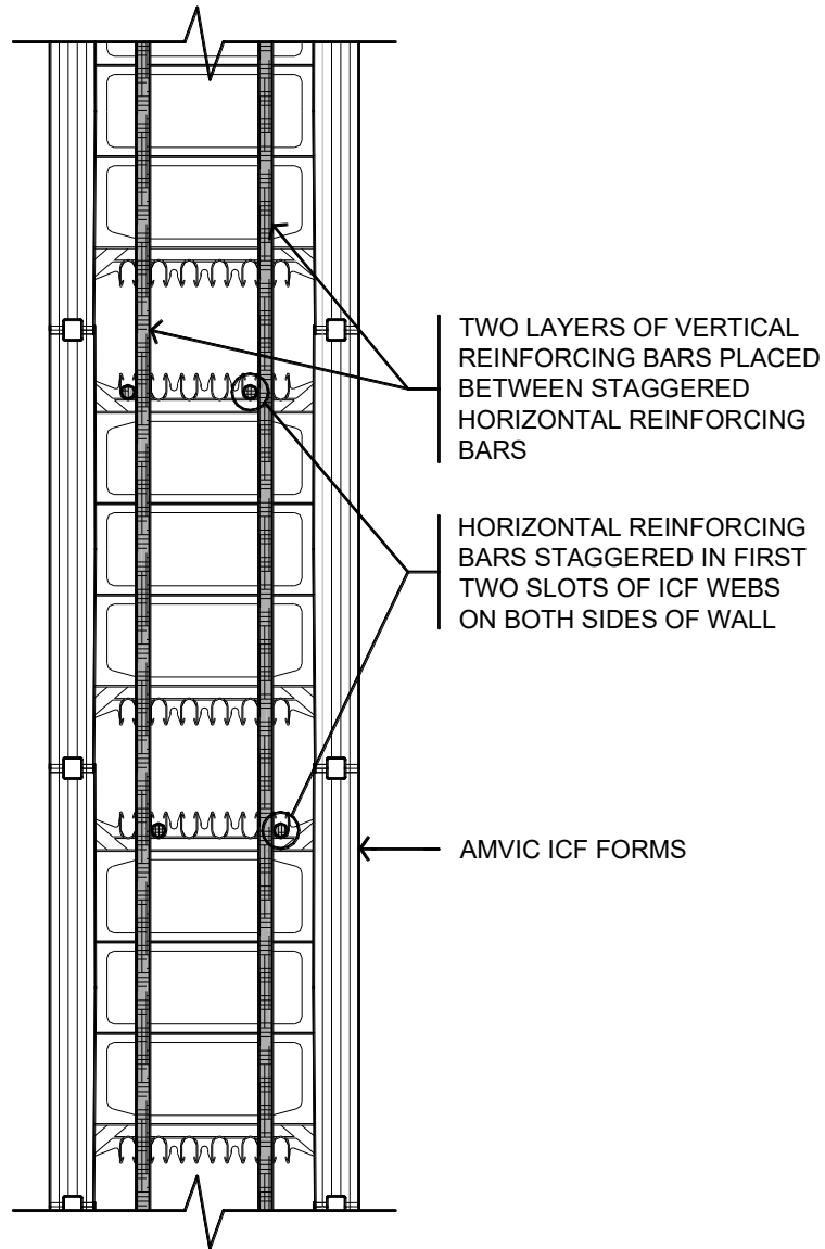
Detail A. 2 – Above grade wall reinforcing placement for 12" thick walls.
