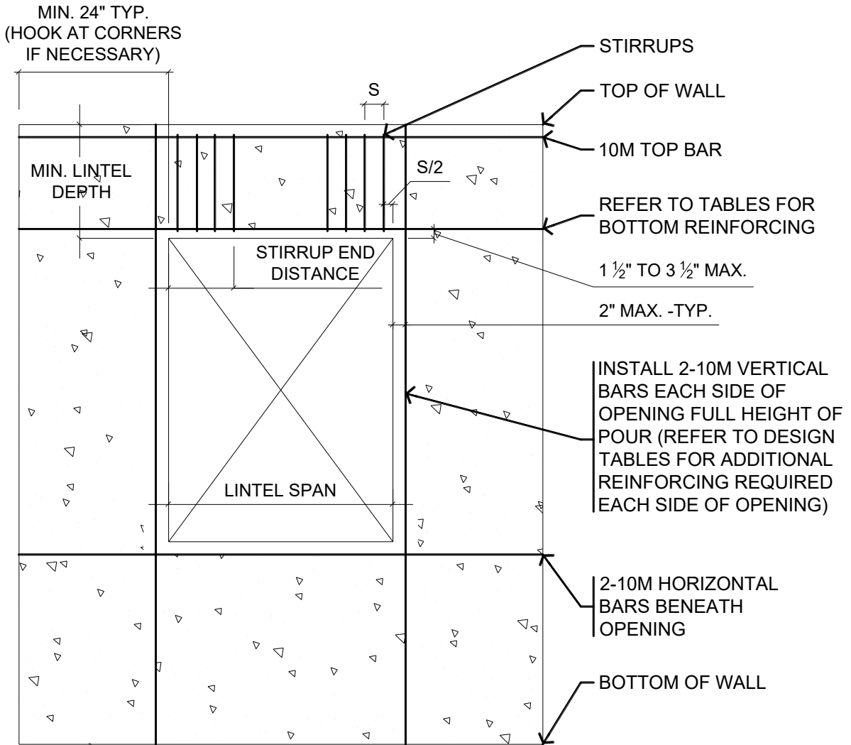
Detail L.1 – Reinforcing around openings.
