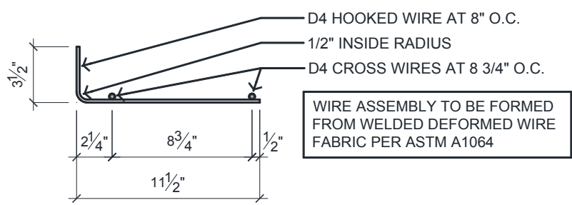
Amvic R30 Brick Ledge Reinforcer
