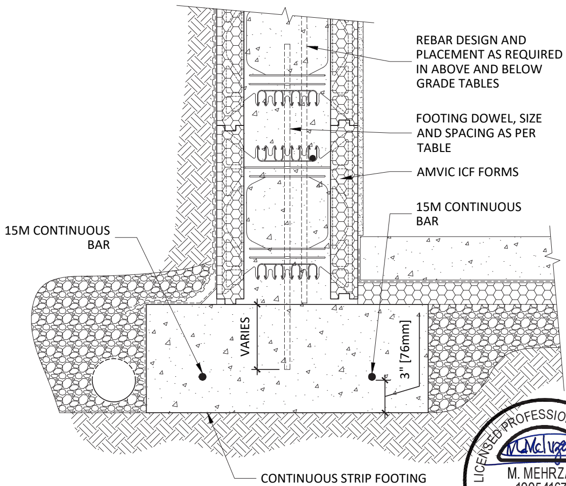
Detail F.1 – Footing dowel detail
