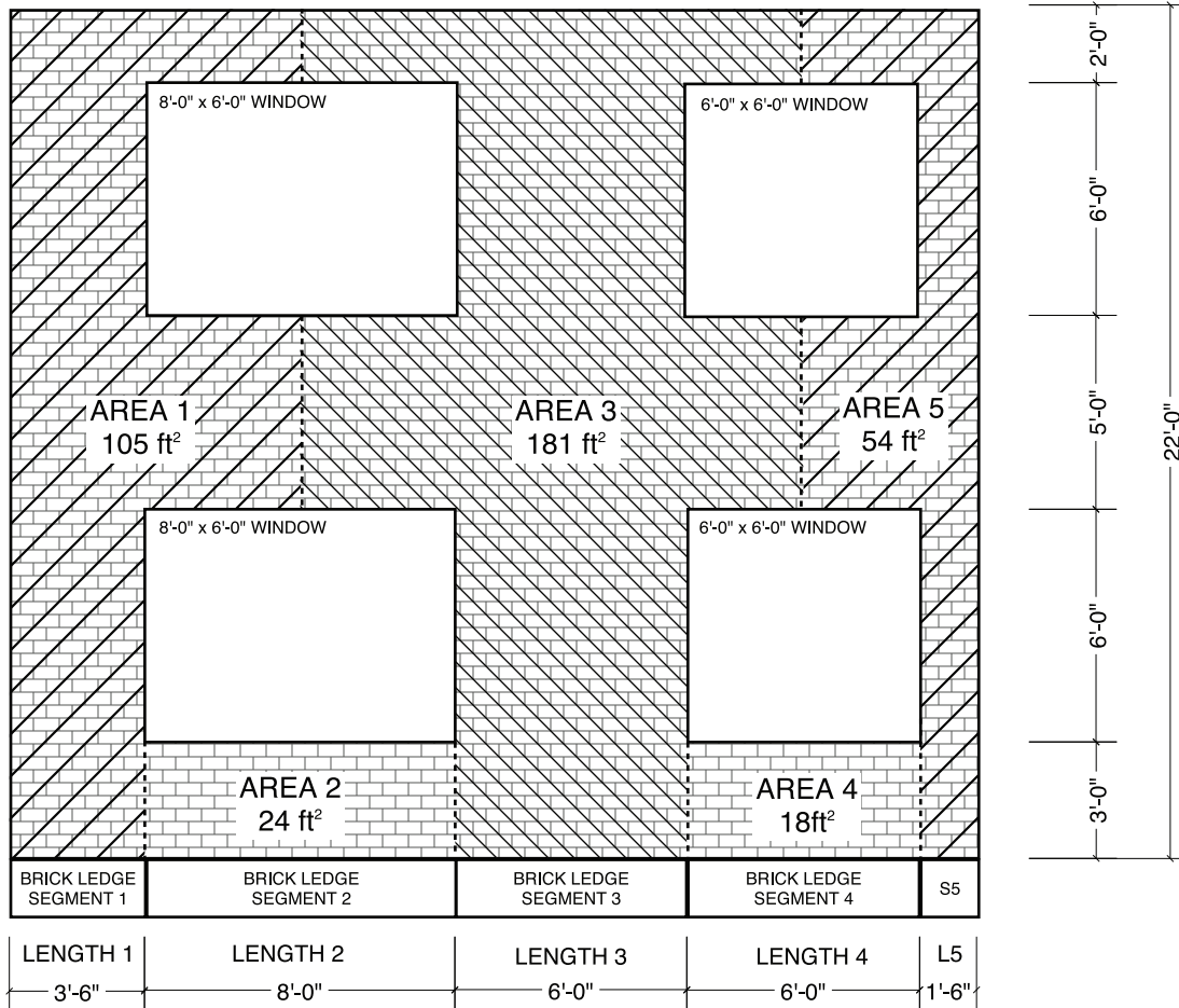
Detail C.2 Masonry veneer area calculation diagram
