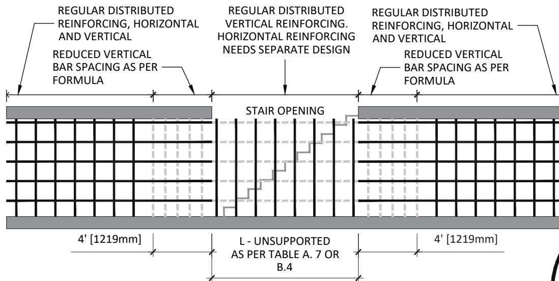
Stair Opening Rebar Diagram
