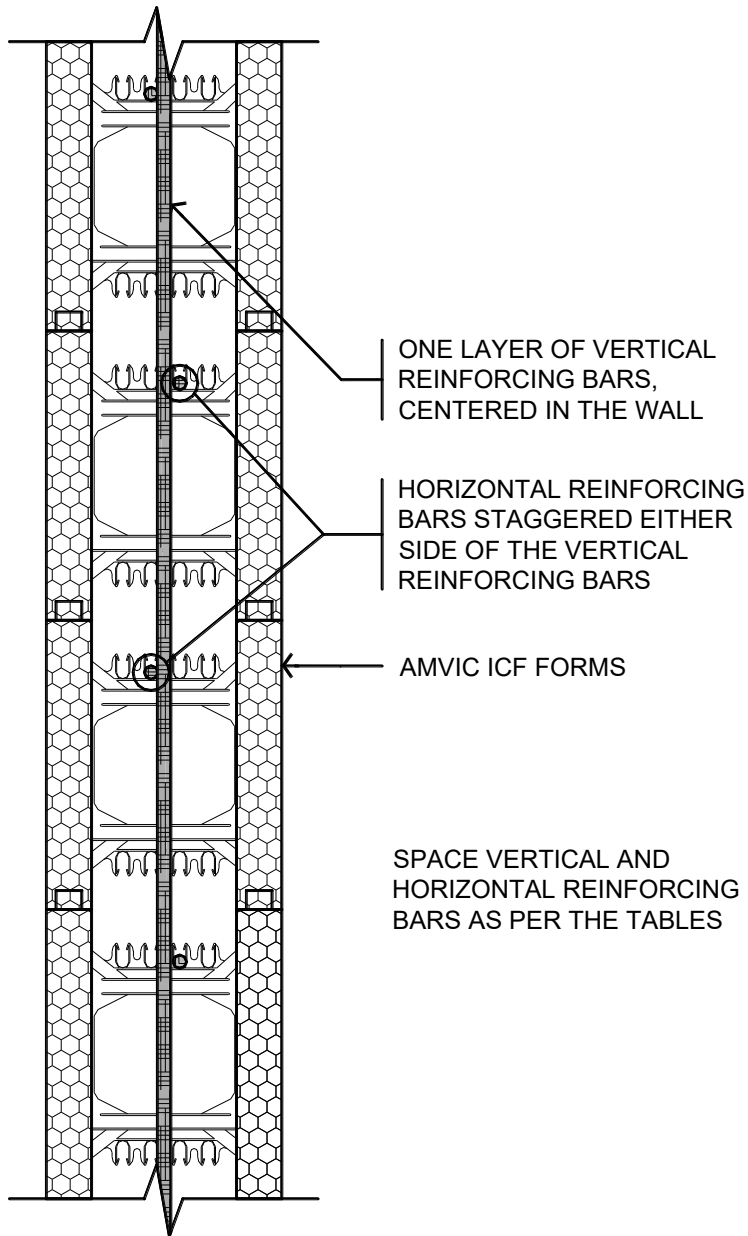
Detail A. 1 – Above grade wall reinforcing placement for 4", 6", 8" and 10" thick walls.
