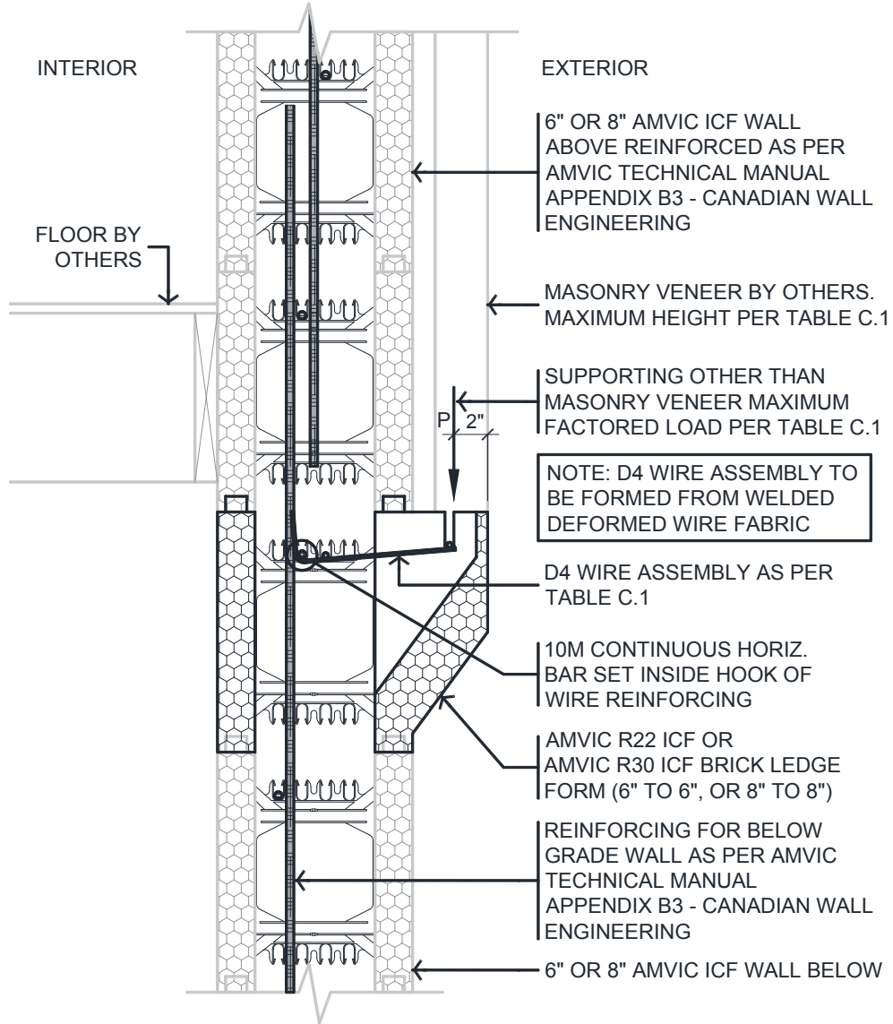
Detail C.1 Brick ledge section
