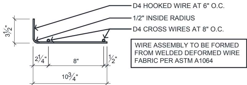
Amvic R22 Brick Ledge Reinforcer
