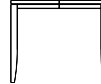
912-706 COUNTER HEIGHT PUB TABLE - RTA W42 D42 H36 (107 x 107 x 91cm) 1-20" (51cm) Leaf, Extends to 62" (157cm). Pages: 14/15
