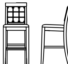
912-692 BAR HEIGHT STOOL - KD W19 D21 H46 (48 x 53 x 117cm) Seat H30 (76cm) Pages: 16/17
