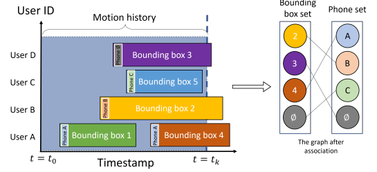
Figure 6: An example of bipartite matching at time t_k . Small vertical boxes overlaid on horizontal boxes denote ground truth associations. The edge weights are computed over the motion history from t_0 to t_k . The algorithm associates bounding box 4 with Phone A, bounding box 2 with Phone B. Bounding box 3 is associated with " \emptyset " to indicate that the user's phone is not opt-in. Phone C is associated with " \emptyset " because its user is not in the camera's field of view.
