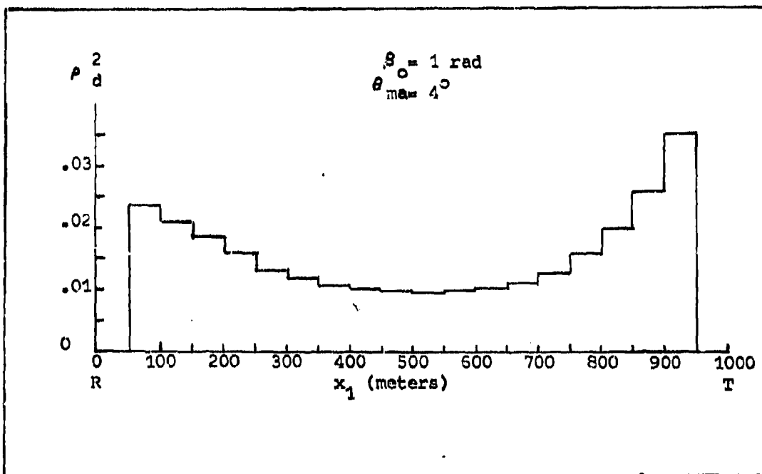
Figure 16. Characteristics of Glistening Area for \beta_0 = 1 rad, R = 1000 m, \theta_{ma} = 4^\circ
