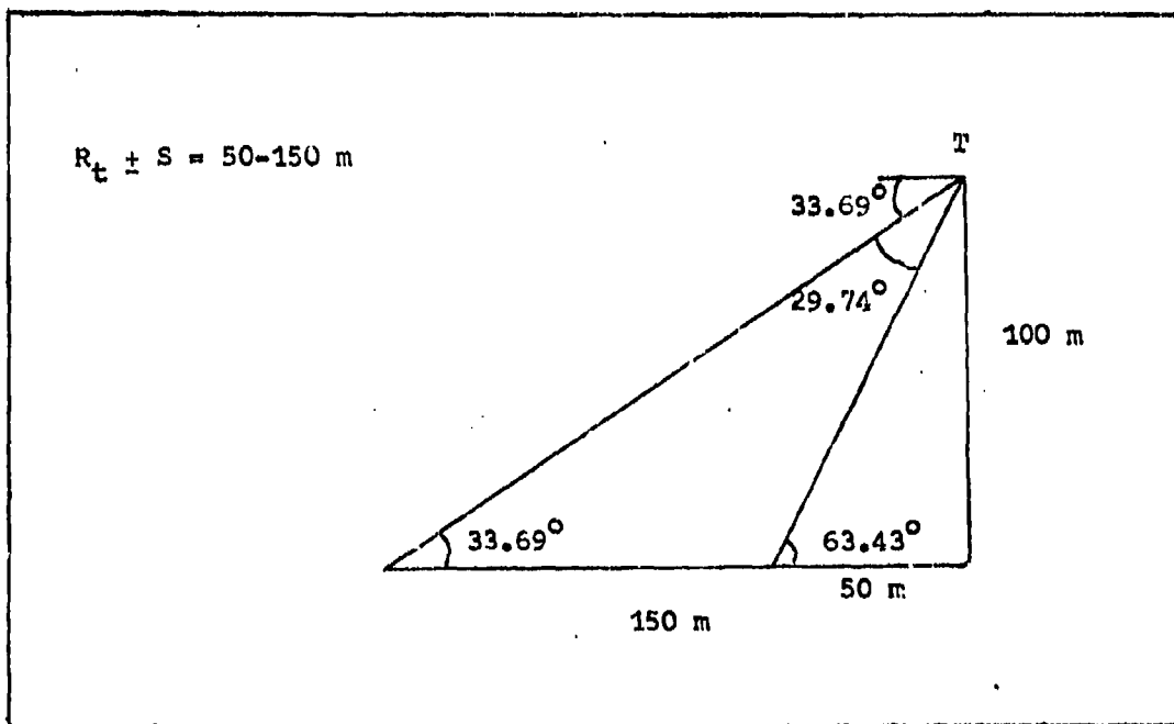
Figure 17. Illumination of Ground Patch for \beta_0 = 1 rad
