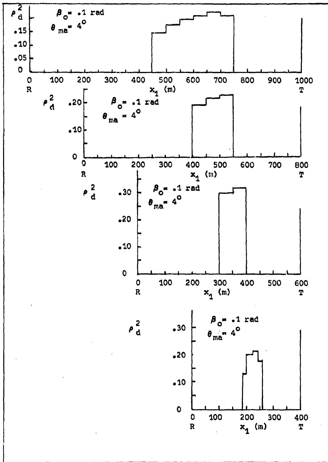
Figure 18. Characteristics of Glistening Area for \beta_0 = .1 rad, Varying Range, \theta_{ma} = 4^\circ
