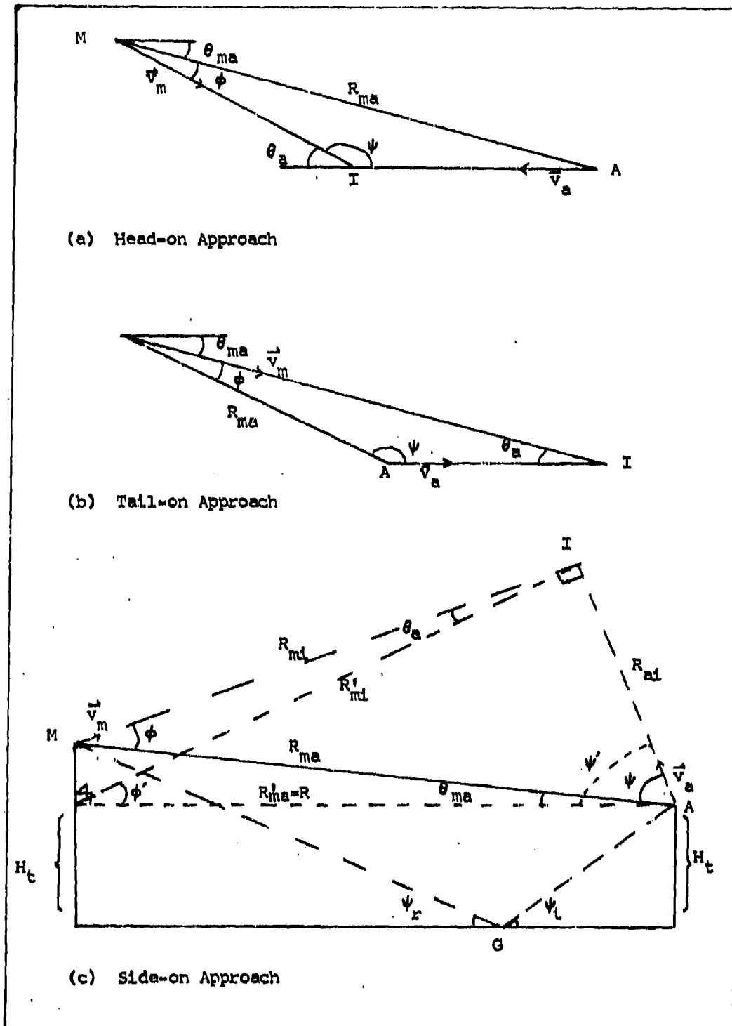
Figure 15. Missile Approach to Target
