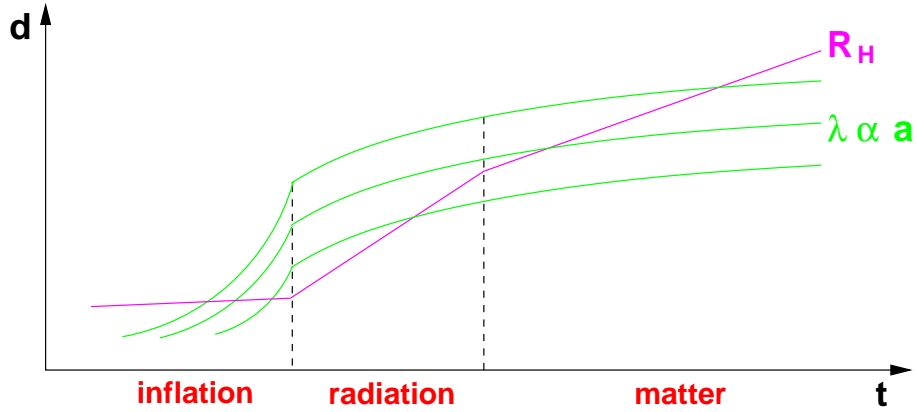
Figure 2.19: Comparison of the Hubble radius with the physical wavelength of a few cosmological perturbations. During the initial stage of accelerated expansion (called inflation), the Hubble radius grows more slowly than each wavelength. So, cosmological perturbations find their origin inside R_H . Then, each mode exits from the Hubble radius during inflation and re-enters during radiation or matter domination.
