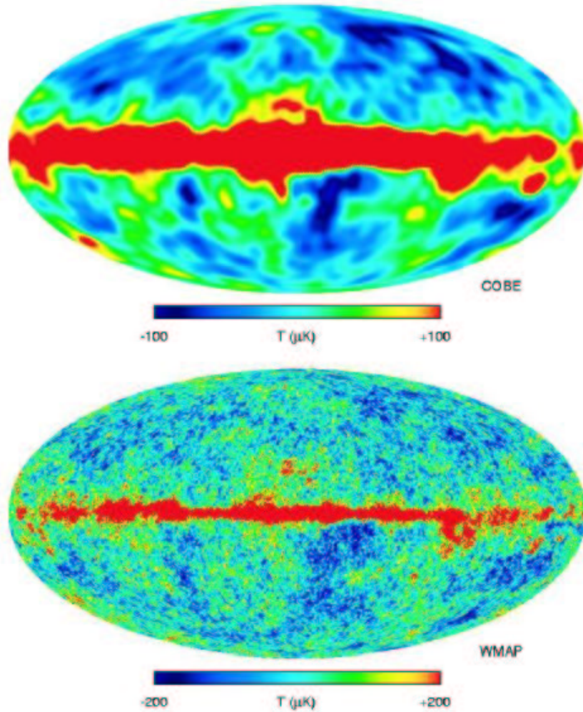
Figure 2.13: Comparison between the COBE and WMAP anisotropy maps. In both figure, the red stripe in the middle is the foreground contamination from the Milky Way. The orientation of the two maps is the same in order to allow for direct visual comparison. The resolution of WMAP is 30 times better, but it is clear that on large angular scale, the two maps reveal the same structure.
