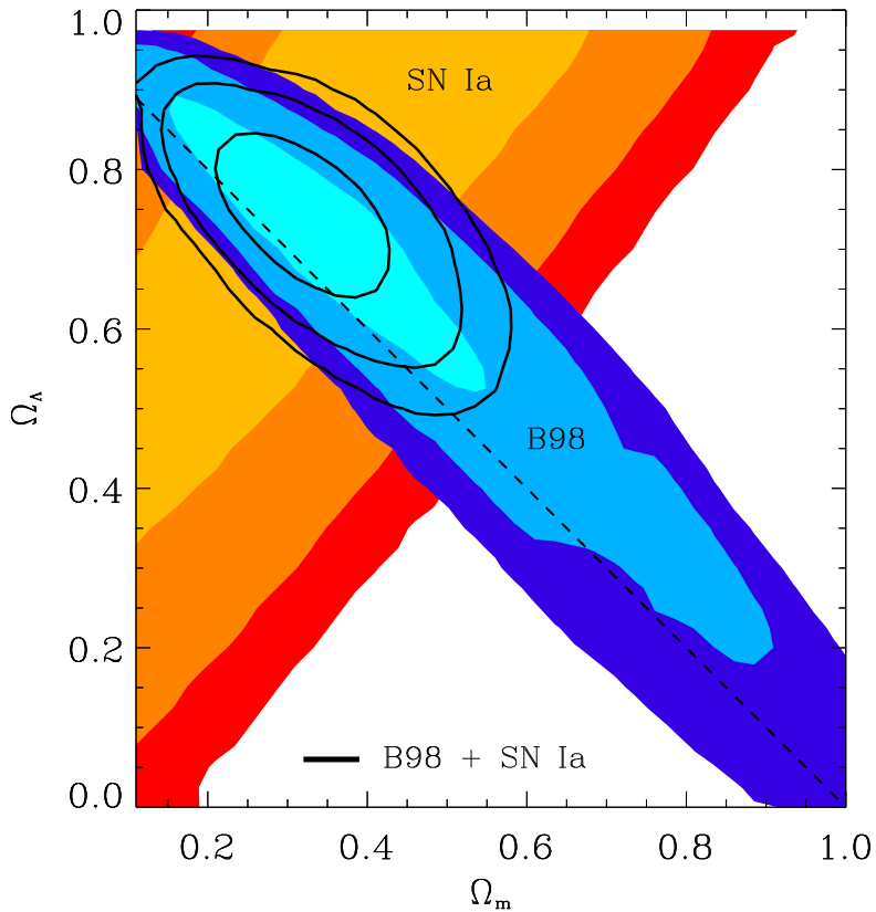
Figure 2.18: Combined constraints on (\Omega_M, \Omega_\Lambda) from CMB and Supernovae experiments. The simple case of a spatially flat Universe with no cosmological constant corresponds to the lower right corner of the plot. In blue, the CMB allowed region favors a spatially flat Universe with \Omega_M + \Omega_\Lambda \simeq 1 . In orange, the Supernovae constraint is orthogonal to the CMB one. By combining the two results, one obtains the favored region limited by the black ellipses, centered near (\Omega_M, \Omega_\Lambda) = (0.3, 0.7) .
