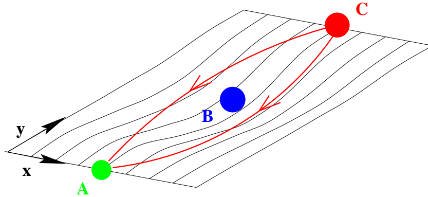
Figure 1.8: Gravitational lensing. Somewhere between an object C and a terrestrial observer A , a massive object B - for instance, a galaxy - curves its surrounding space-time. Here, for simplicity, we only draw two spatial dimensions. In absence of gravity and curvature, the only possible trajectory of light between C and A would be a straight line. But because of curvature, the straight line is not anymore the shortest trajectory. Photons prefer to follow two geodesics, symmetrical around B . So, the observer will not see one image of C , but two distinct images. In fact, if we restore the third spatial dimension, and if the three points are perfectly aligned, the image of C will appear as a ring around B . This phenomenon is observed in practice.
