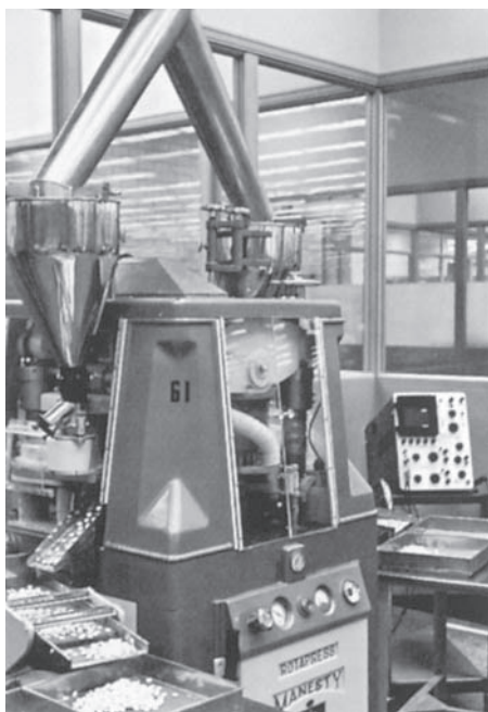
FIGURE 8.25 Manesty Rotapress rotary compression machine. Tablets leaving the machine run over a tablet duster to screen, where they are inspected. Material to be compressed is fed from the overhead hopper through yoke to the two compressing machine hoppers. Hardness of tablet is monitored electronically by oscilloscope at right. (Courtesy of Upjohn Company.)
