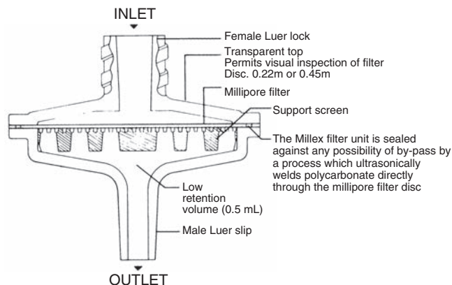
FIGURE 15.6 Cutaway showing composition of the Milllex filter unit. (Courtesy of Millipore Corporation.)
