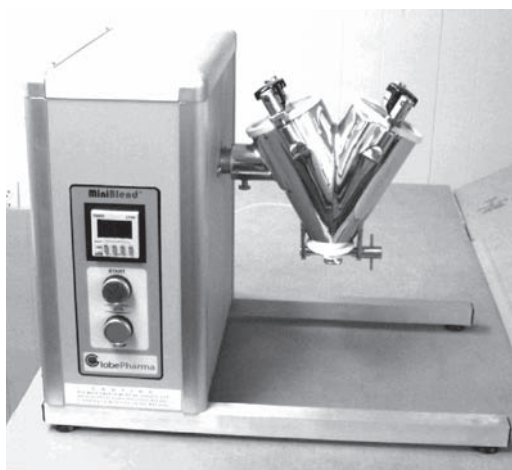
FIGURE 6.4 Laboratory-scale V-blender. (Courtesy of Globepharm.)
