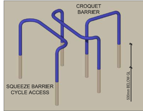
B Isometric of Squeeze Barrier 001
