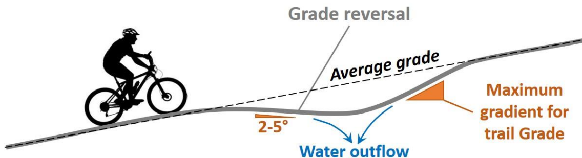
Figure 22: Typical grade reversal (not to scale)
