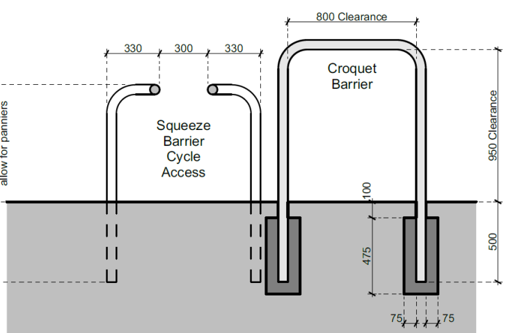
E Section through c/l of squeeze barriers 001 not to a particular scale
