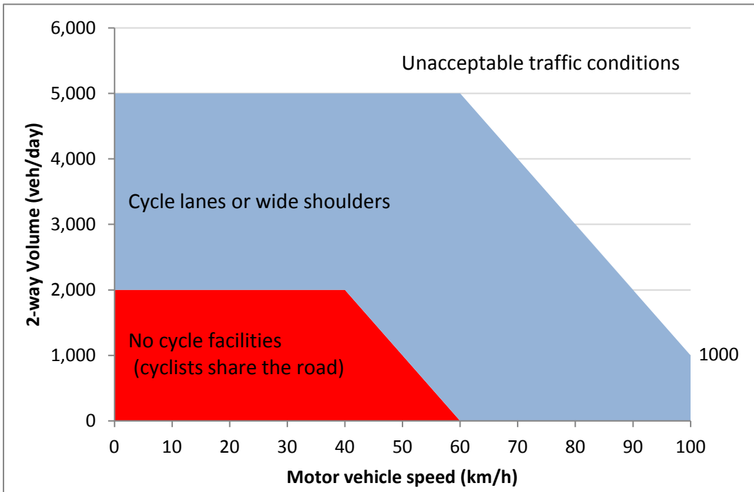
Figure 45: Trail type for Grade 1 and 2 on-road trails
