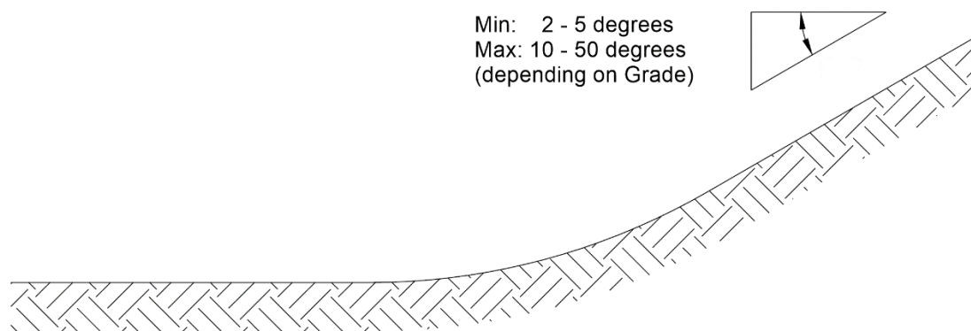
Figure 23: Cross section for super-elevated (or bermed) turns
