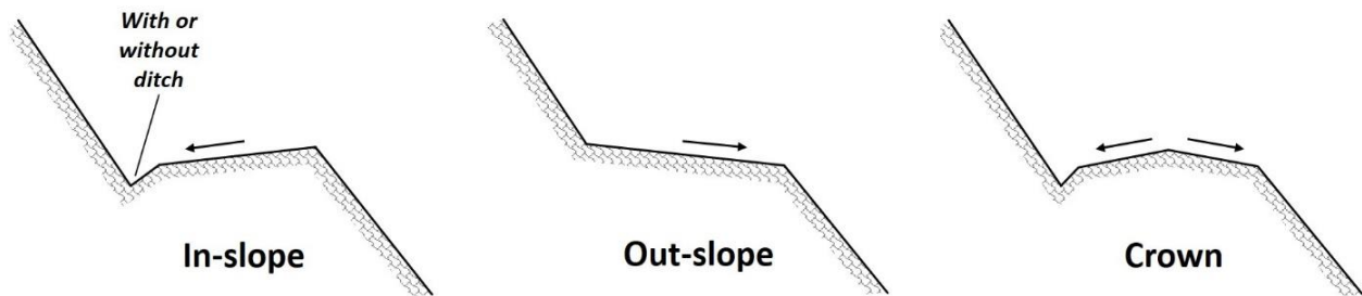
Figure 24: Different options for trail cross-sections
