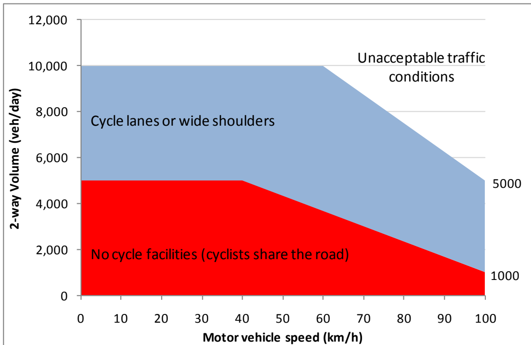
Figure 46: Trail type for Grade 3 and 4 on-road trails
