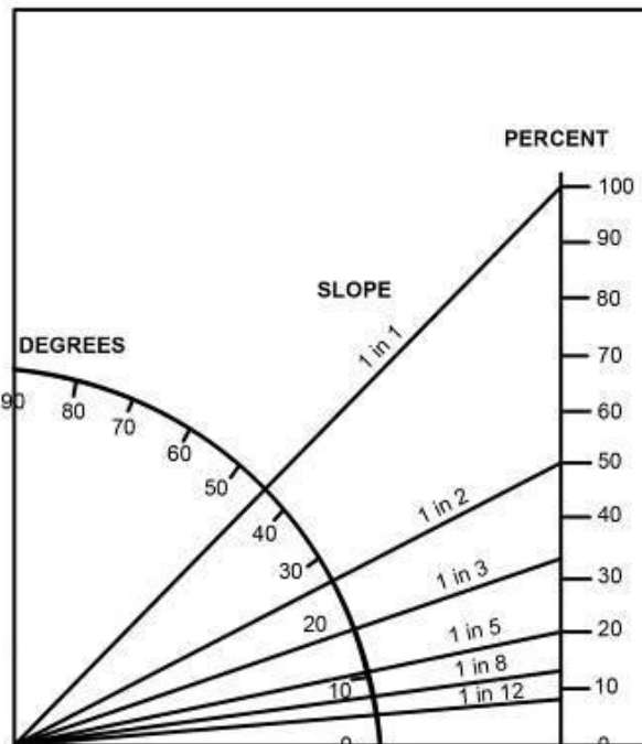
Figure 17: Relationship between degrees, percent and slope
