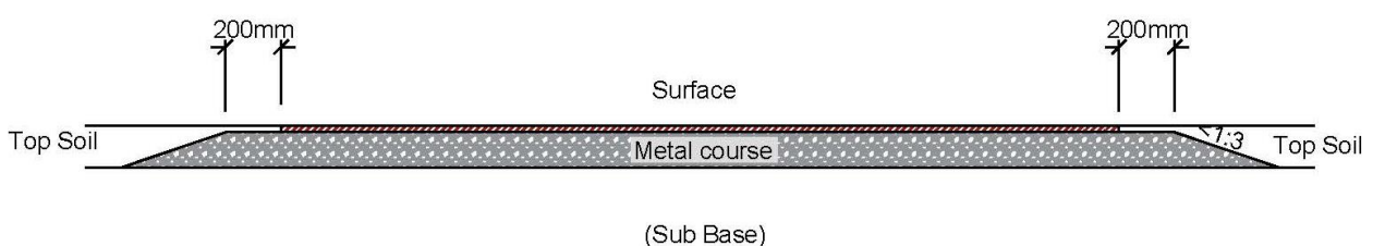
Figure 32: Cross section for chipseal or AC path without timber edging battens
