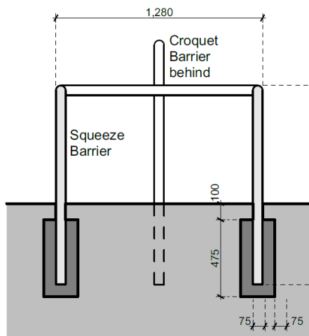
D Elevation of squeeze barrier 001 not to a particular scale
