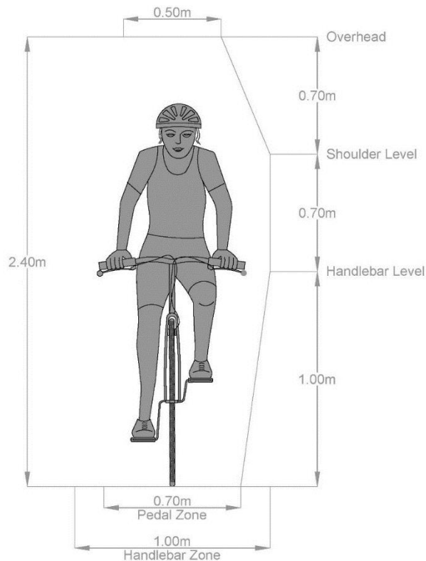
Figure 20: Cycle operating space
