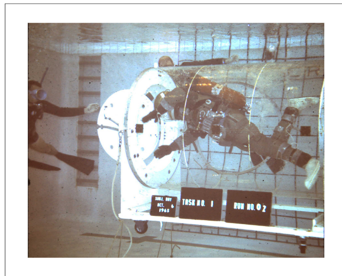
Figure 3. Neutral Buoyancy test in the McDonogh pool with the NASA Langley airlock mockup, October 1965. Courtesy of Sam Mattingly.
