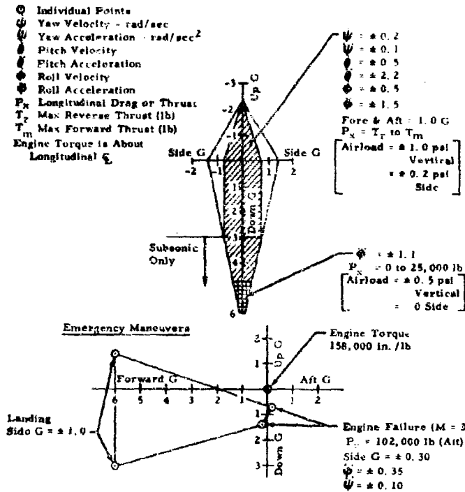
Figure 8. JTF17 Maneuver Load Diagram - Lockheed Installation
