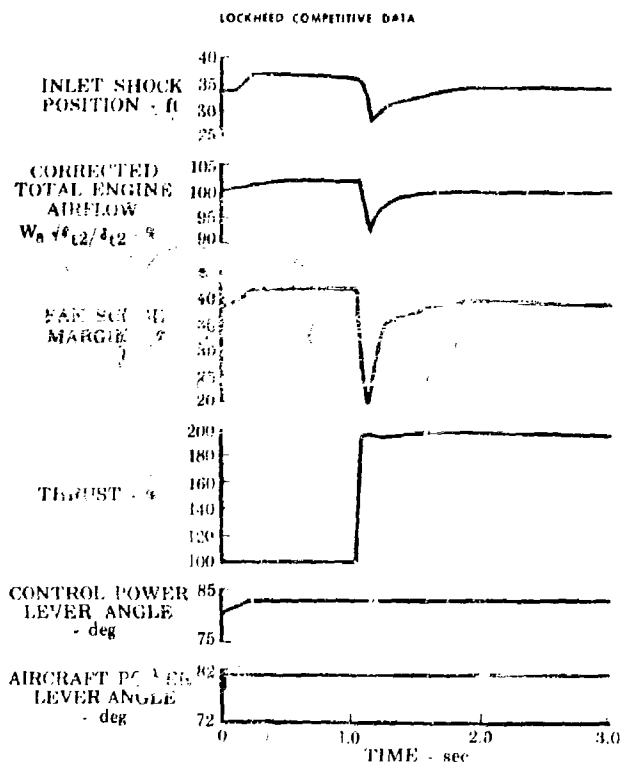
Figure 25. JTF17 Cruise Phase II-B Minimum Duct Heater Lightoff (F/A = 0.008) PD 16715 DII
