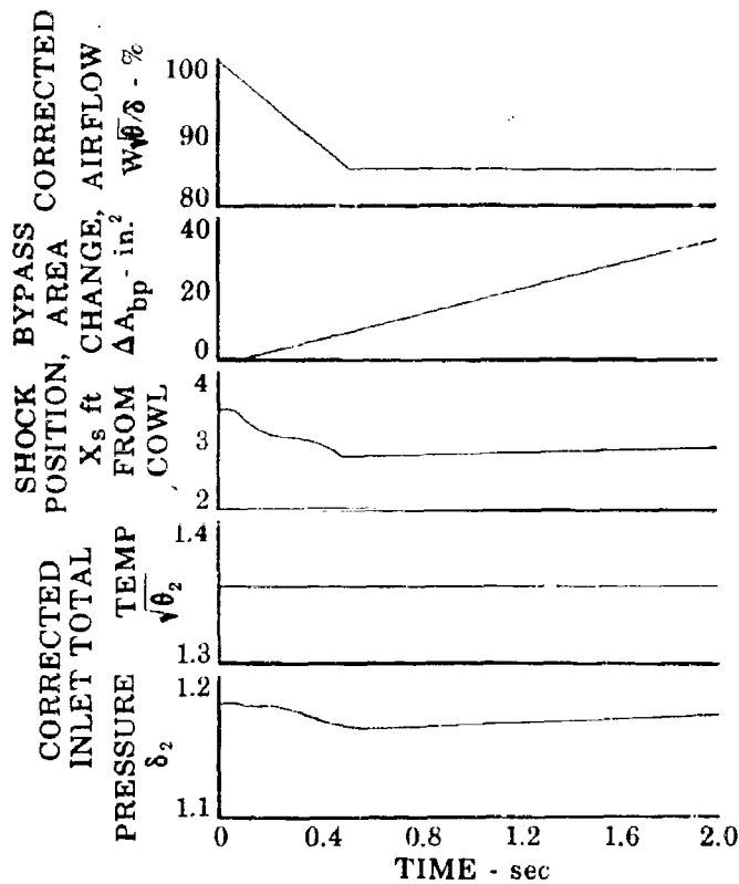
Figure 33. Inlet Response to Change in Corrected Flow F1 16745
