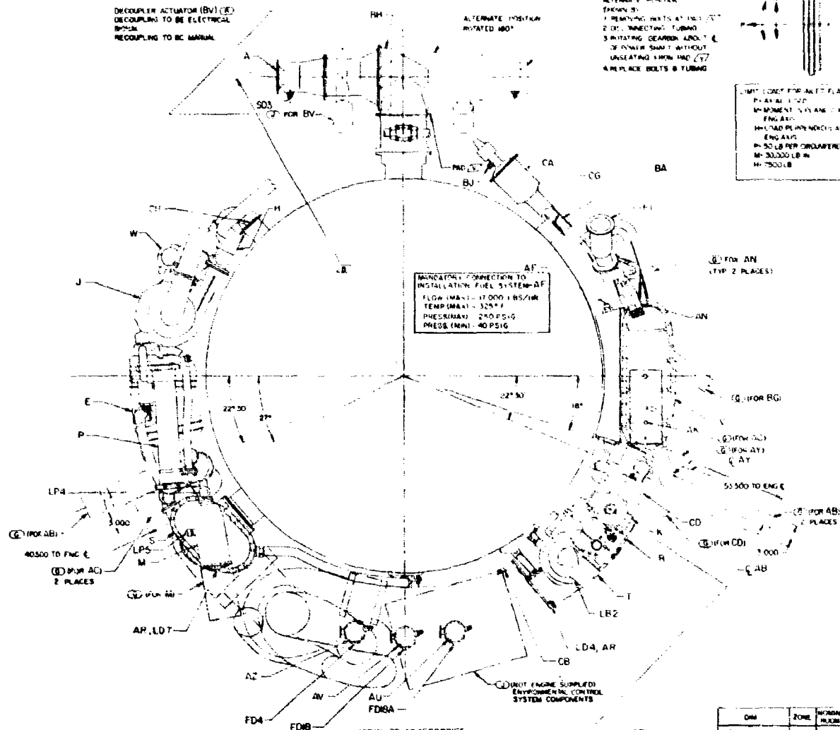
VIEW OF ACCESSORIES VIEWED FROM INLET END
