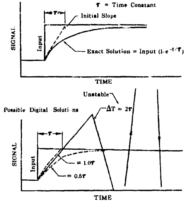
Figure 7. Stability Criterion for Digital Programming of Dynamic Simulations FD 16692 DII
