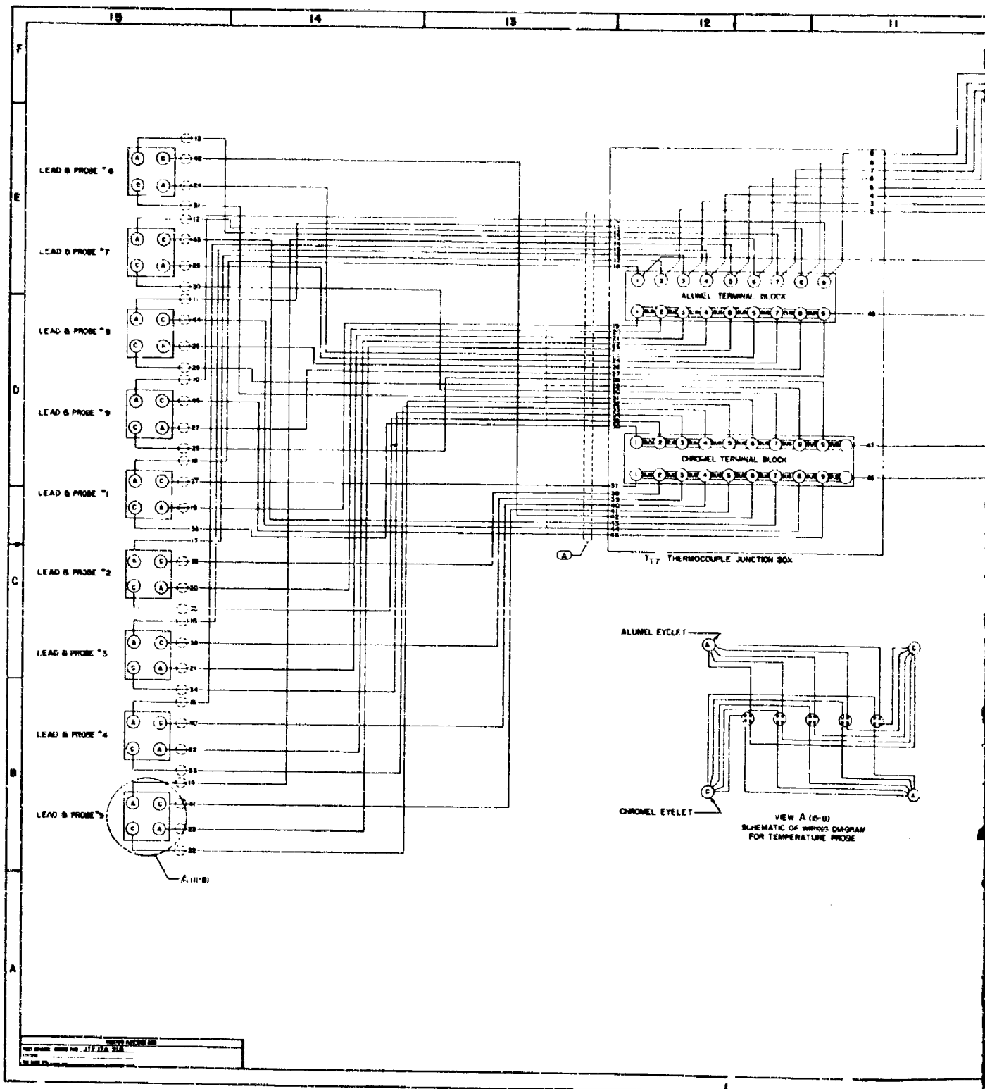
Figure 6. Diagram, Electrical Installation Connection (Boeing)
