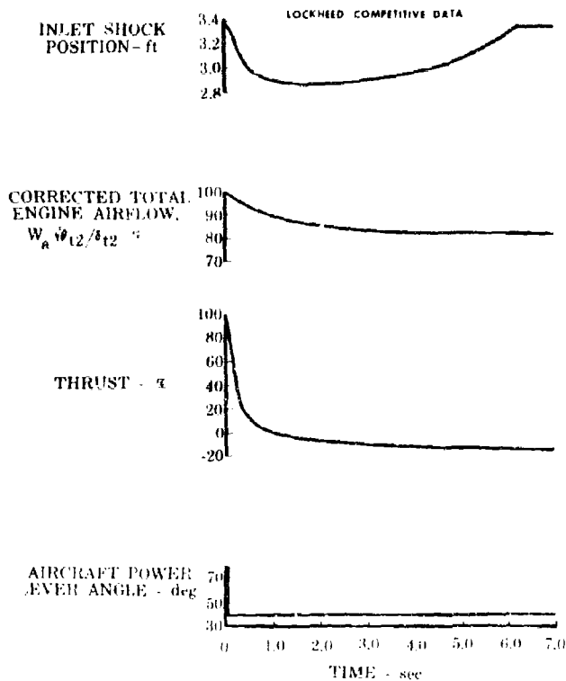
Figure 34. JTF17 Cruise Maximum Nonaugmented to Idle FD 16718 DII
