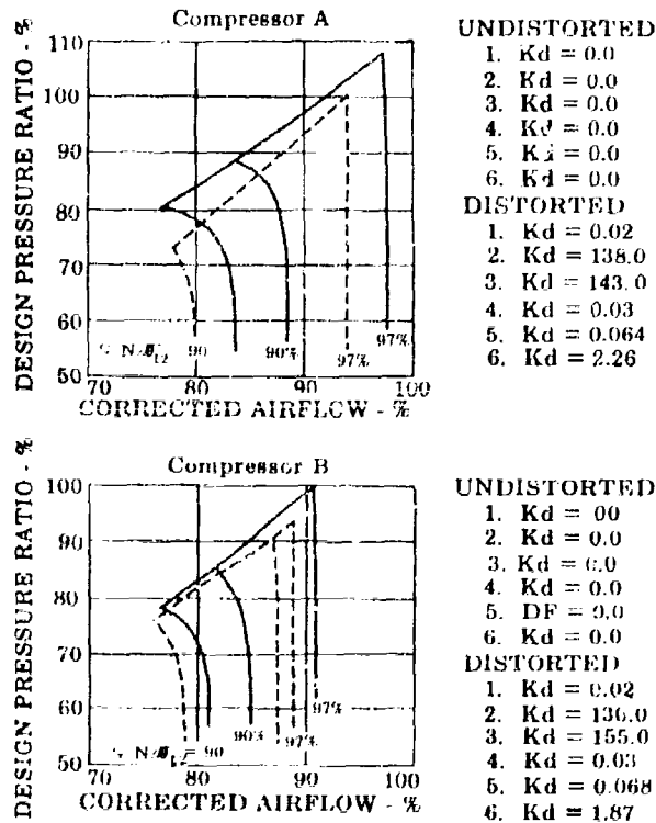
Figure 38. Effect of a Specific Distortion On Two Compressors
