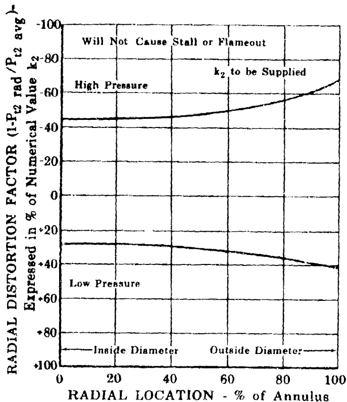
Figure 48. Estimated Limiting Value of Radial Component of Inlet Total Pressure Distortion - Will Not Cause Stall or Flameout FD 17821 DTT
