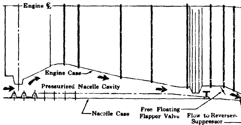
Figure 7. Lockneed Secondary Air Flow System
