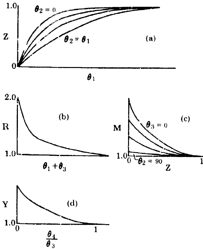
Figure 51. Slope and Response Factors to be Used in Intermixing "Blade Element" Distortion Limits FD 17804 DII
