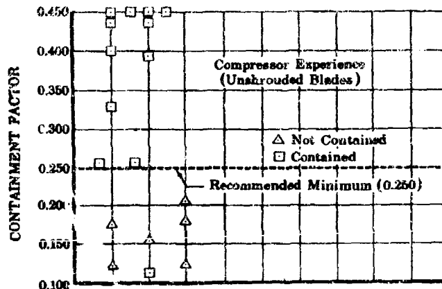
Figure 25. Containment Experience
