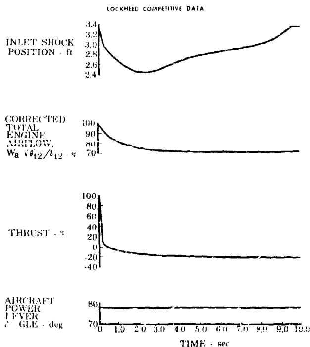
Figure 36. JTF17 Cruise Maximum Nonaugmented Fuel Shutoff Valve Turned Off - Engine Windmills FD 16719 DII
