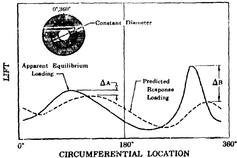
Figure 43. Predicted Rotor Blade Response
