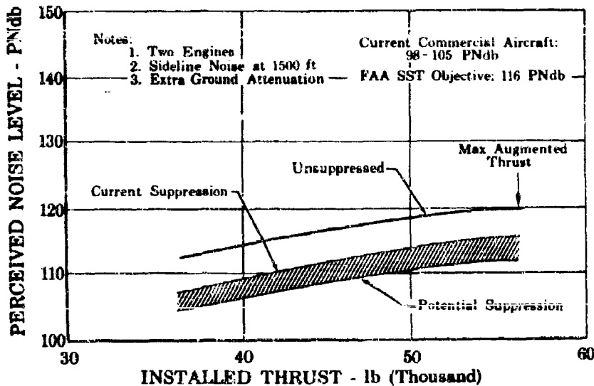
Figure 15. Predicted Turbofan Airport Noise Levels FD 16948
