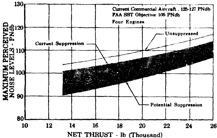
Figure 16. Predicted Turbofan Noise Levels at Thrust Cutback After Takeoff FD 16949
