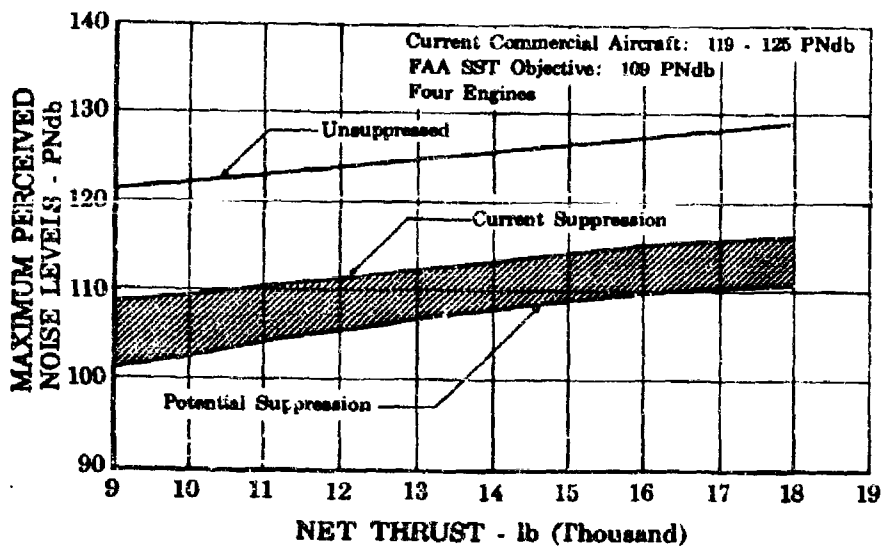
Figure 17. Predicted Turbofan Noise Levels at Approach Conditions FD 16950
