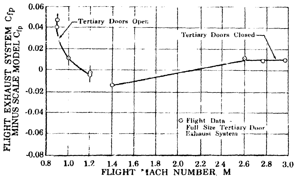
Figure 2. Performance Comparison of Flight and Scale Model Exhaust Systems FD 17100 DIII
