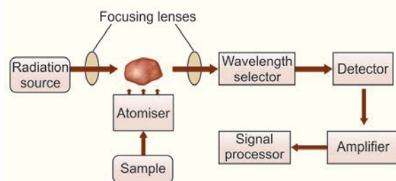
Fig 36.6: Atomic absorption spectrophotometry
