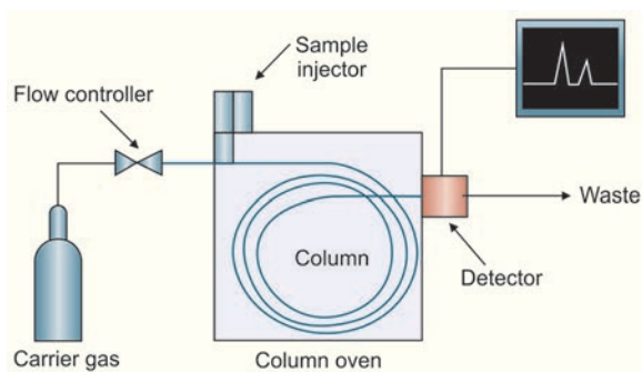
Fig 36.3: Gas chromatography
